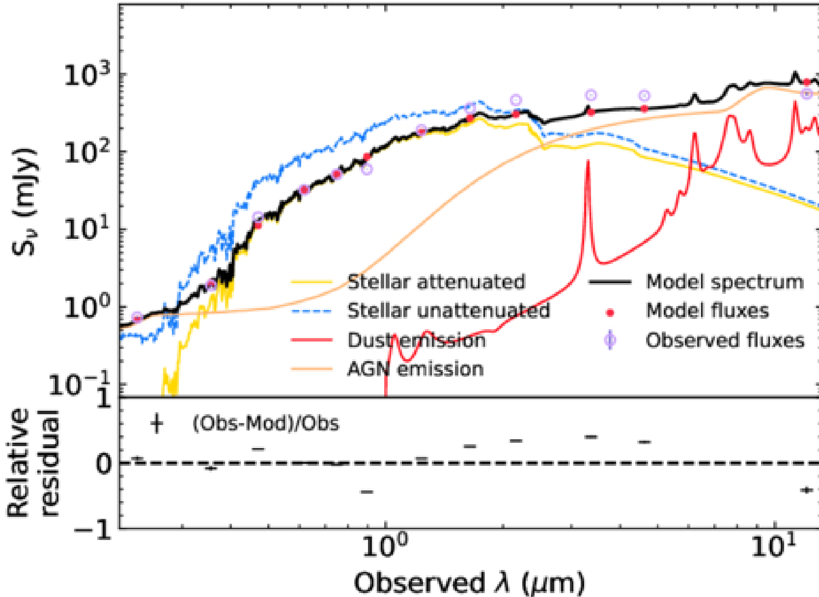
Figure 15. from Dezheng Meng et al 2026 Astrophys. J. 1002 doi:10.3847/1538-4357/ae4c87 https://dx.doi.org/10.3847/1538-4357/ae4c87 © 2026. The Author(s). Published by the American Astronomical Society.
