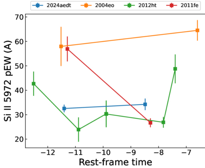
Figure 14. from Dezheng Meng et al 2026 Astrophys. J. 1002 doi:10.3847/1538-4357/ae4c87 https://dx.doi.org/10.3847/1538-4357/ae4c87 © 2026. The Author(s). Published by the American Astronomical Society.
