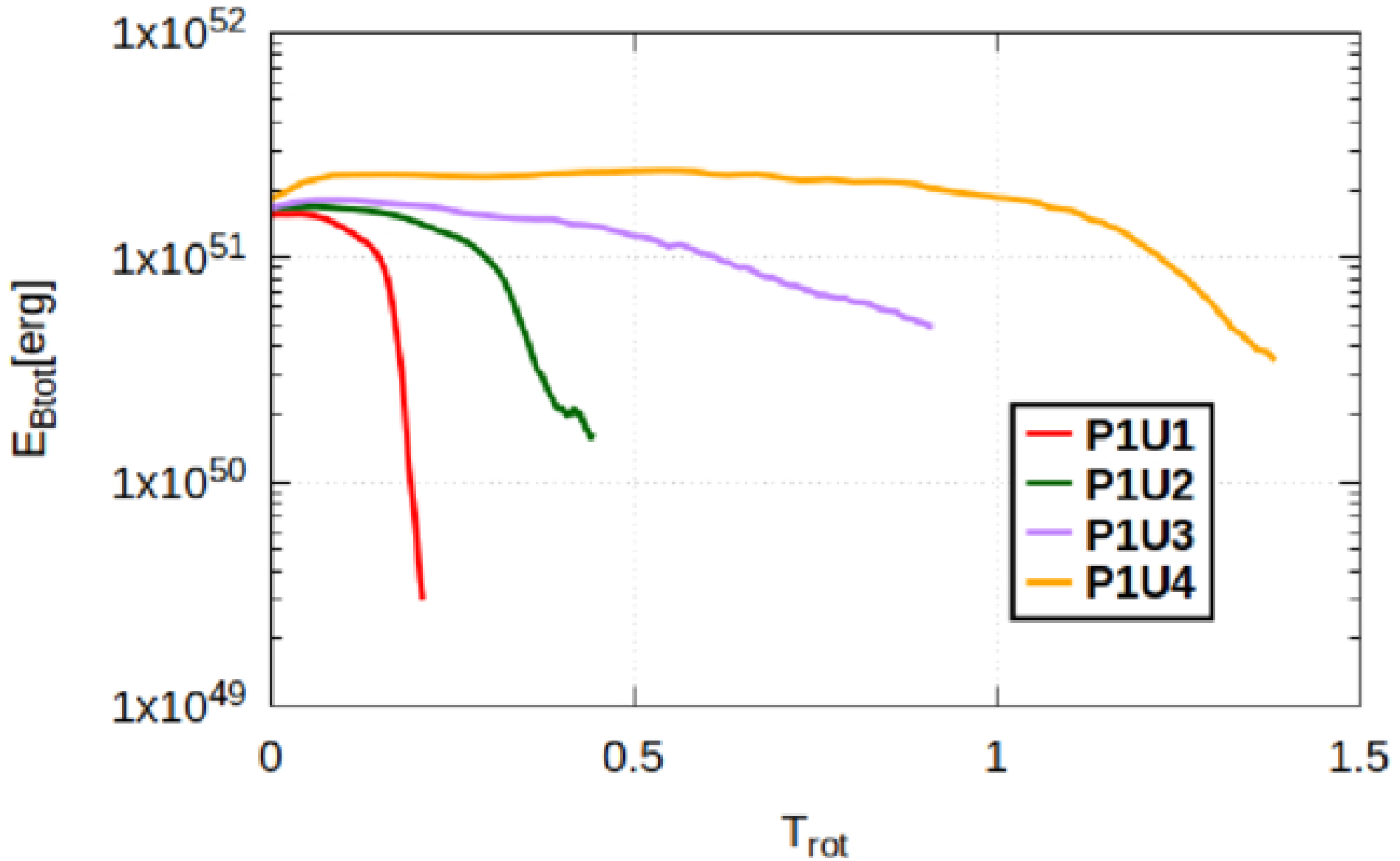
Figure 9. from Fabrizio Venturi Piñas et al 2026 Astrophys. J. 1001 doi:10.3847/1538-4357/ae4c3f https://dx.doi.org/10.3847/1538-4357/ae4c3f © 2026. The Author(s). Published by the American Astronomical Society.
