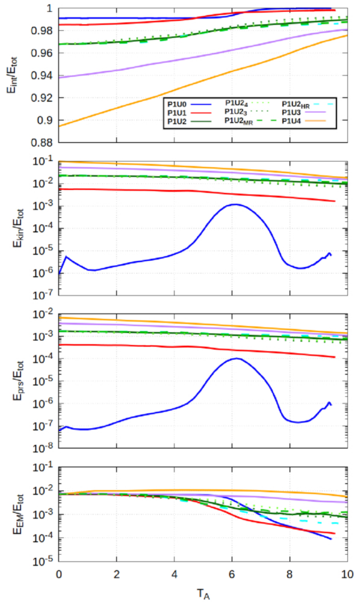
Figure 8. from Fabrizio Venturi Piñas et al 2026 Astrophys. J. 1001 doi:10.3847/1538-4357/ae4c3f https://dx.doi.org/10.3847/1538-4357/ae4c3f © 2026. The Author(s). Published by the American Astronomical Society.
