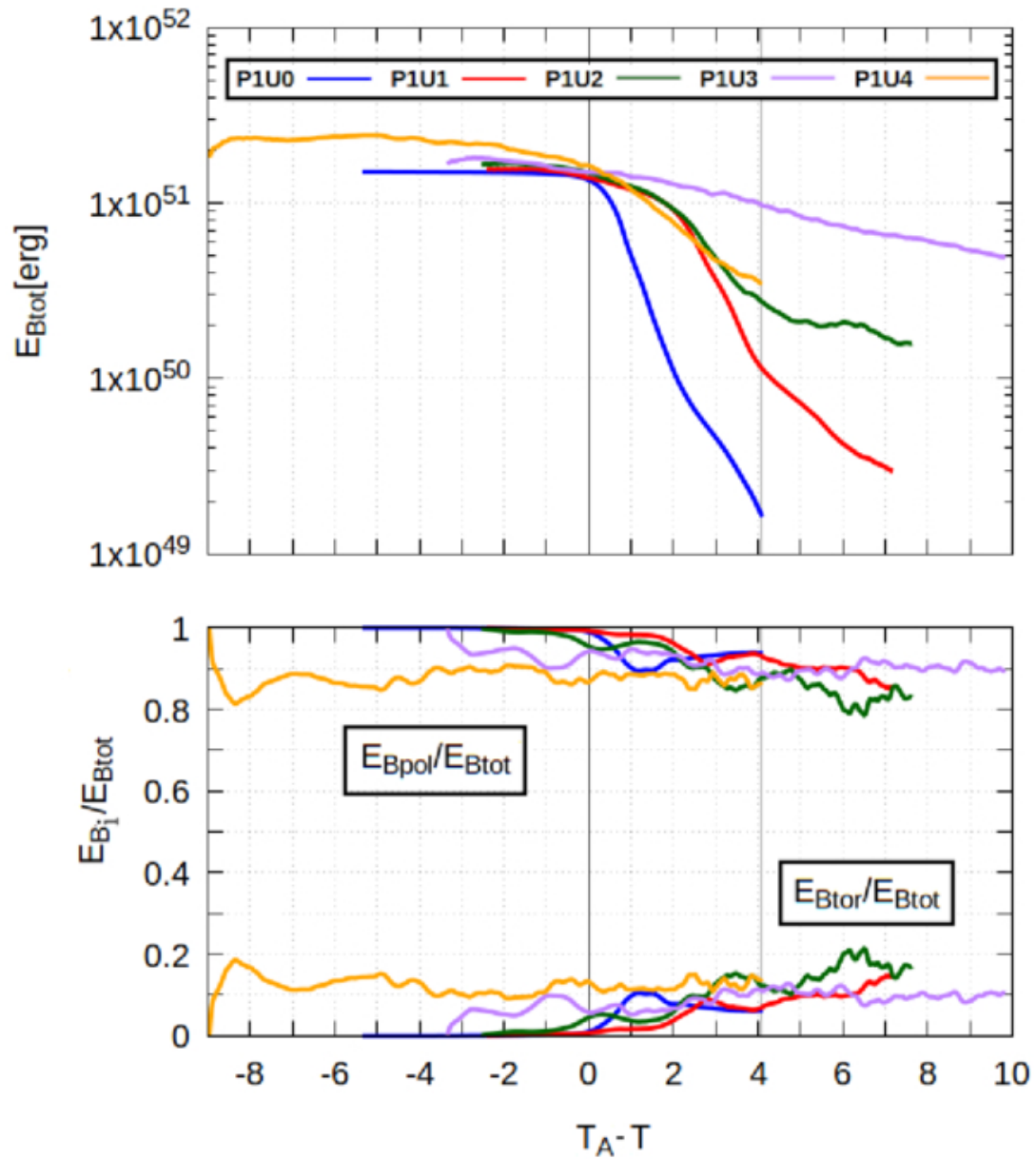
Figure 7. from Fabrizio Venturi Piñas et al 2026 Astrophys. J. 1001 doi:10.3847/1538-4357/ae4c3f https://dx.doi.org/10.3847/1538-4357/ae4c3f © 2026. The Author(s). Published by the American Astronomical Society.
