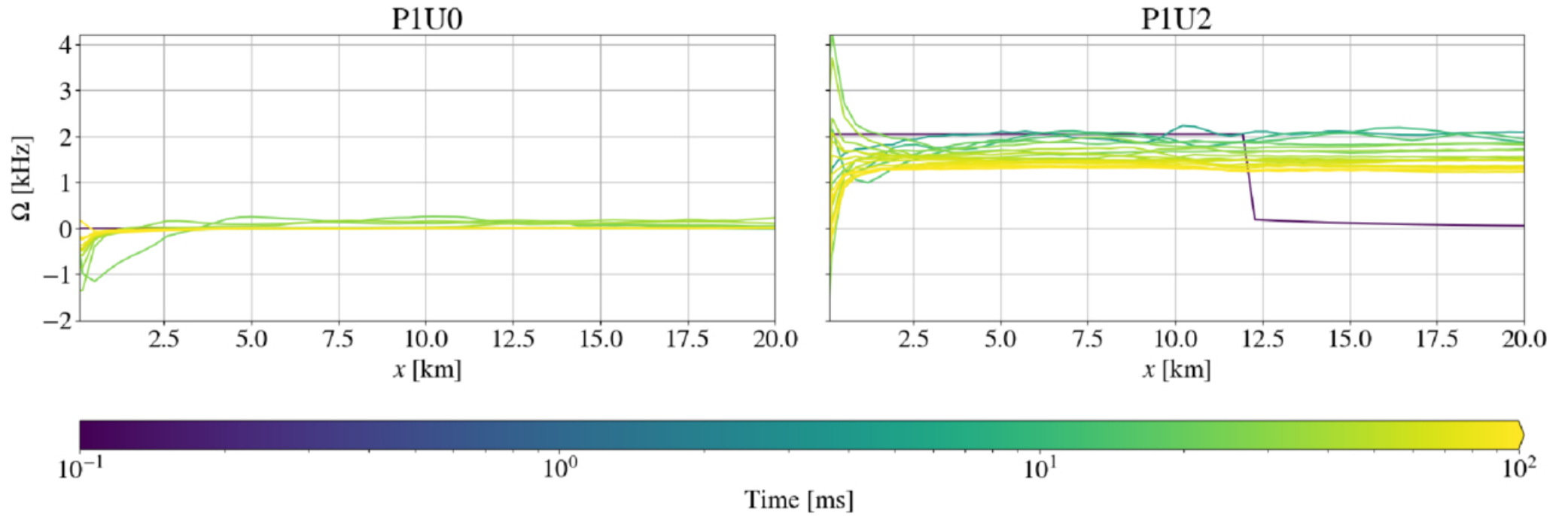
Figure 5. from Fabrizio Venturi Piñas et al 2026 Astrophys. J. 1001 doi:10.3847/1538-4357/ae4c3f https://dx.doi.org/10.3847/1538-4357/ae4c3f © 2026. The Author(s). Published by the American Astronomical Society.
