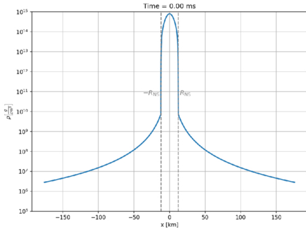
Figure 2. from Fabrizio Venturi Piñas et al 2026 Astrophys. J. 1001 doi:10.3847/1538-4357/ae4c3f https://dx.doi.org/10.3847/1538-4357/ae4c3f © 2026. The Author(s). Published by the American Astronomical Society.
