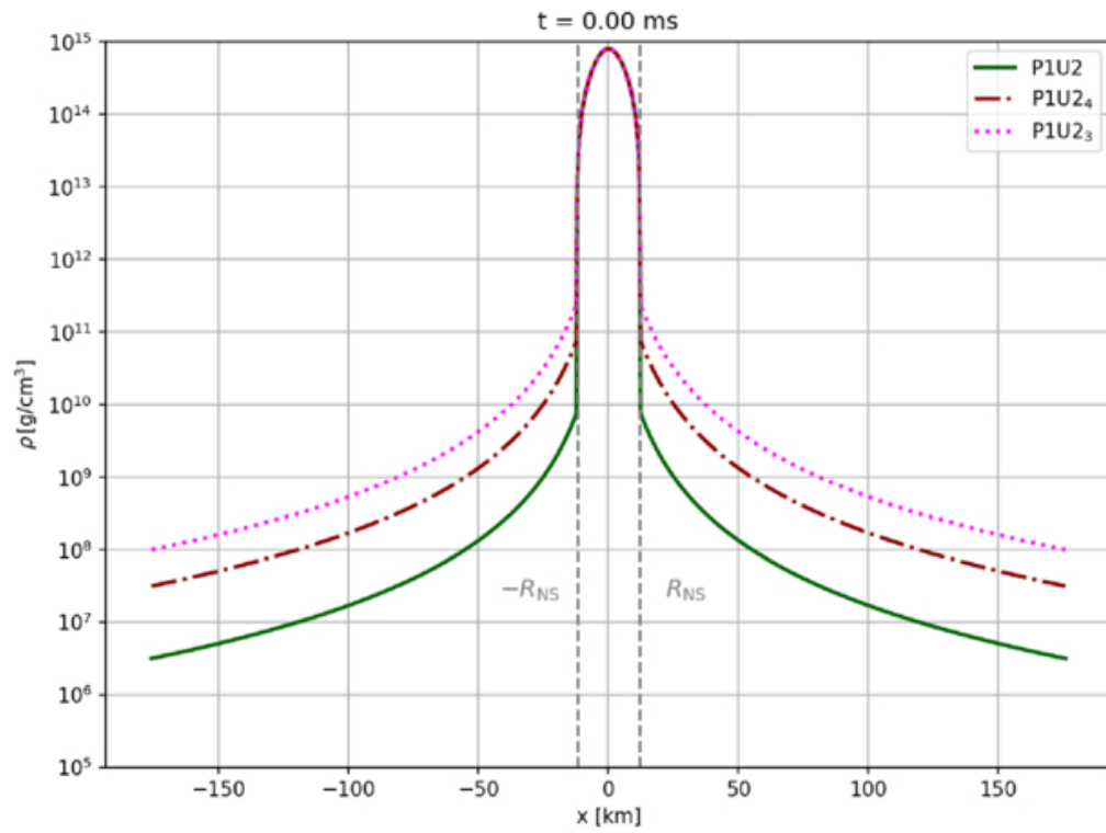
Figure 12. from Fabrizio Venturi Piñas et al 2026 Astrophys. J. 1001 doi:10.3847/1538-4357/ae4c3f https://dx.doi.org/10.3847/1538-4357/ae4c3f © 2026. The Author(s). Published by the American Astronomical Society.
