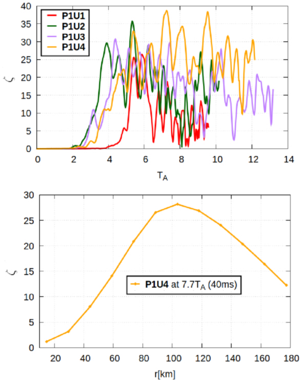
Figure 11. from Fabrizio Venturi Piñas et al 2026 Astrophys. J. 1001 doi:10.3847/1538-4357/ae4c3f https://dx.doi.org/10.3847/1538-4357/ae4c3f © 2026. The Author(s). Published by the American Astronomical Society.
