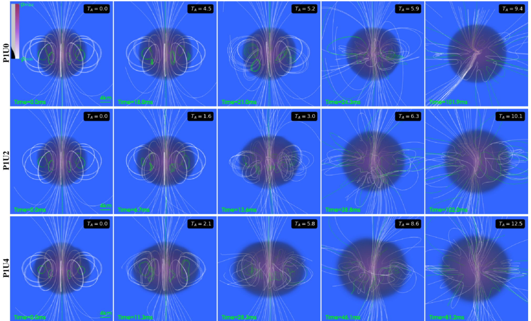
Figure 1. from Fabrizio Venturi Piñas et al 2026 Astrophys. J. 1001 doi:10.3847/1538-4357/ae4c3f https://dx.doi.org/10.3847/1538-4357/ae4c3f © 2026. The Author(s). Published by the American Astronomical Society.
