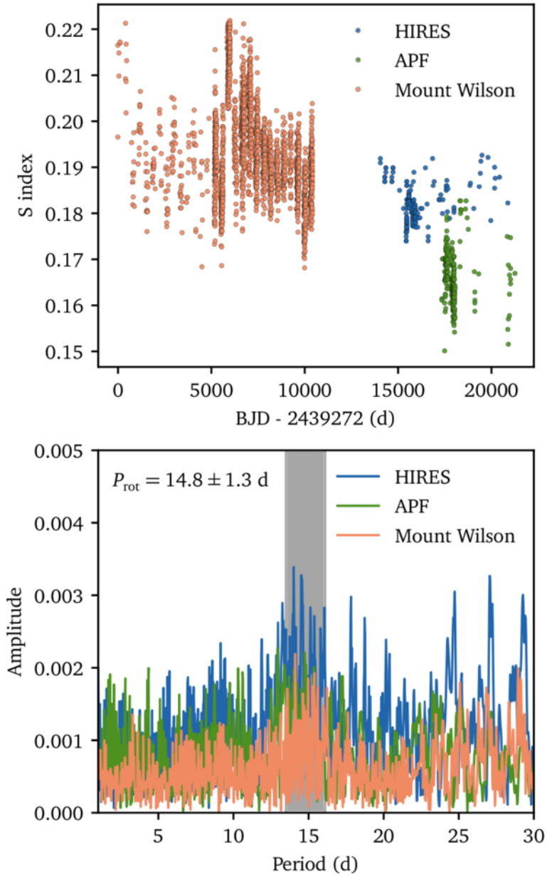
Figure 7. from Yaguang Li et al 2026 Astrophys. J. 1002 doi:10.3847/1538-4357/ae4bdb https://dx.doi.org/10.3847/1538-4357/ae4bdb © 2026. The Author(s). Published by the American Astronomical Society.
