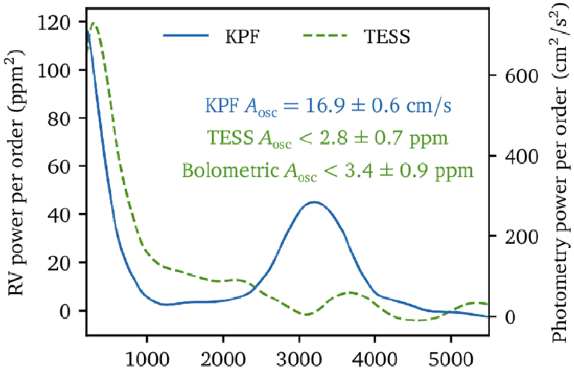
Figure 6. from Yaguang Li et al 2026 Astrophys. J. 1002 doi:10.3847/1538-4357/ae4bdb https://dx.doi.org/10.3847/1538-4357/ae4bdb © 2026. The Author(s). Published by the American Astronomical Society.
