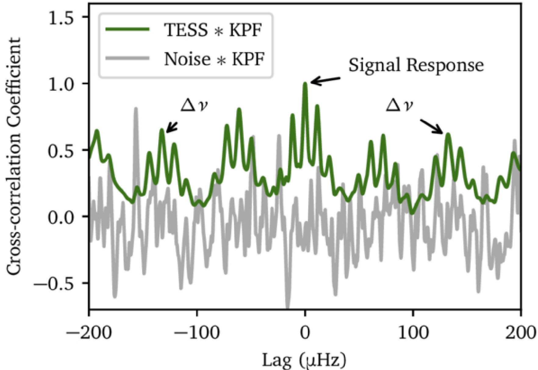
Figure 5. from Yaguang Li et al 2026 Astrophys. J. 1002 doi:10.3847/1538-4357/ae4bdb https://dx.doi.org/10.3847/1538-4357/ae4bdb © 2026. The Author(s). Published by the American Astronomical Society.
