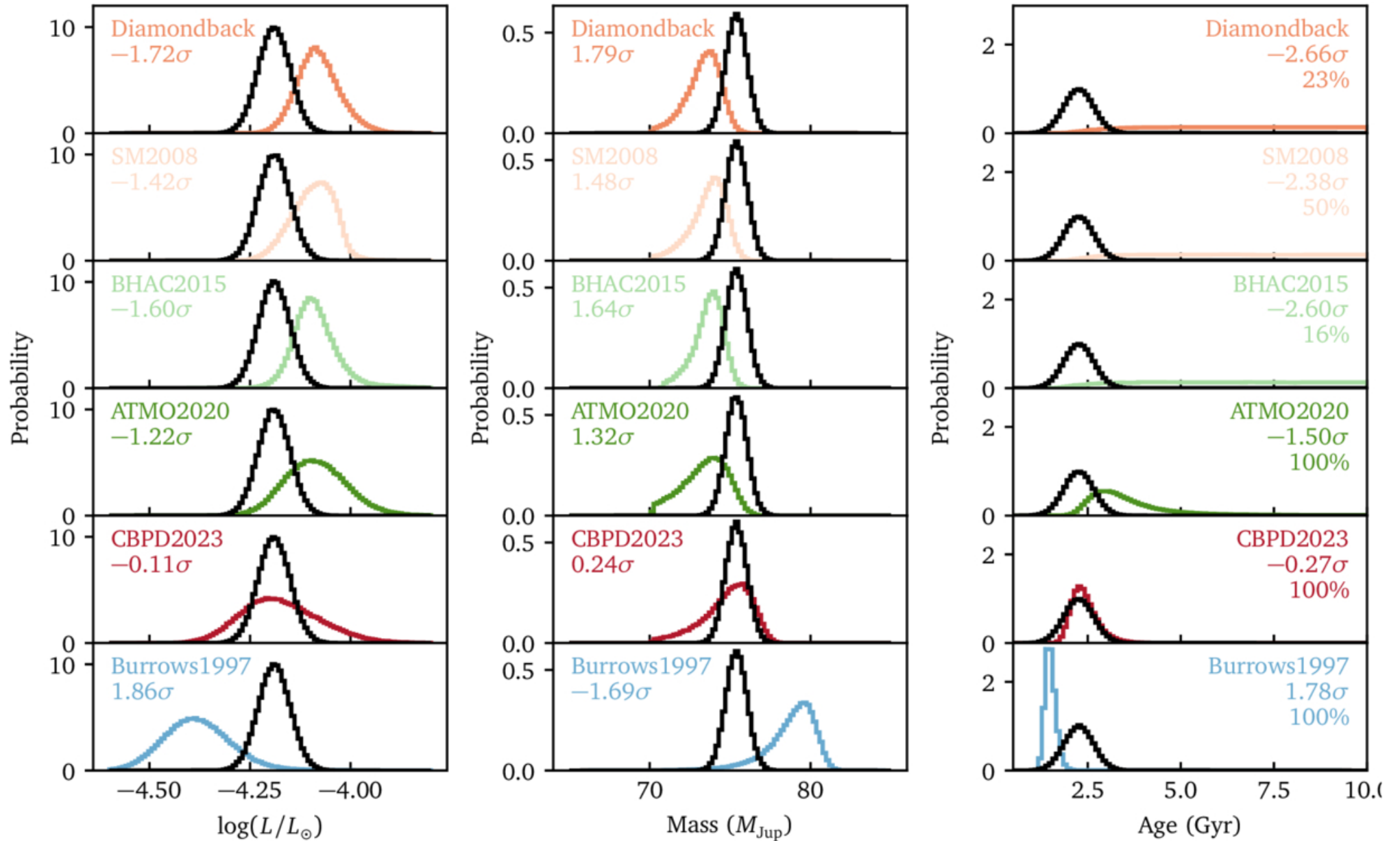
Figure 13. from Yaguang Li et al 2026 Astrophys. J. 1002 doi:10.3847/1538-4357/ae4bdb https://dx.doi.org/10.3847/1538-4357/ae4bdb © 2026. The Author(s). Published by the American Astronomical Society.
