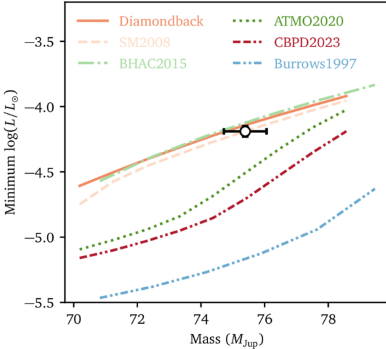
Figure 12. from Yaguang Li et al 2026 Astrophys. J. 1002 doi:10.3847/1538-4357/ae4bdb https://dx.doi.org/10.3847/1538-4357/ae4bdb © 2026. The Author(s). Published by the American Astronomical Society.
