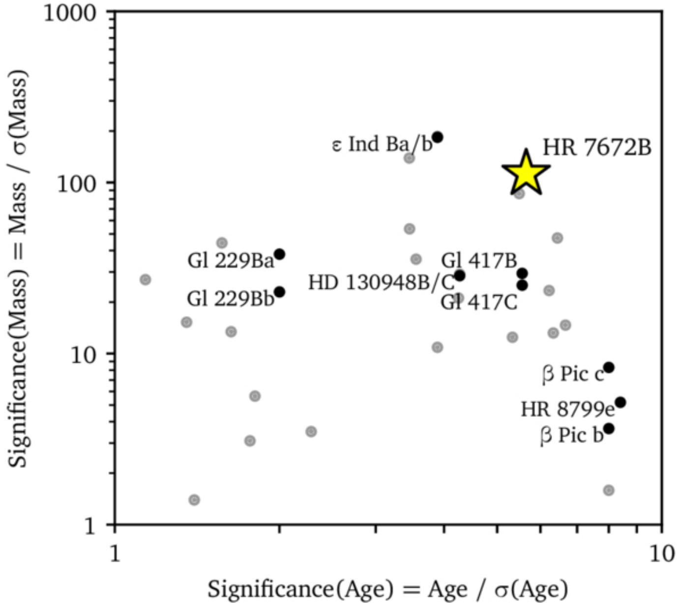
Figure 10. from Yaguang Li et al 2026 Astrophys. J. 1002 doi:10.3847/1538-4357/ae4bdb https://dx.doi.org/10.3847/1538-4357/ae4bdb © 2026. The Author(s). Published by the American Astronomical Society.
