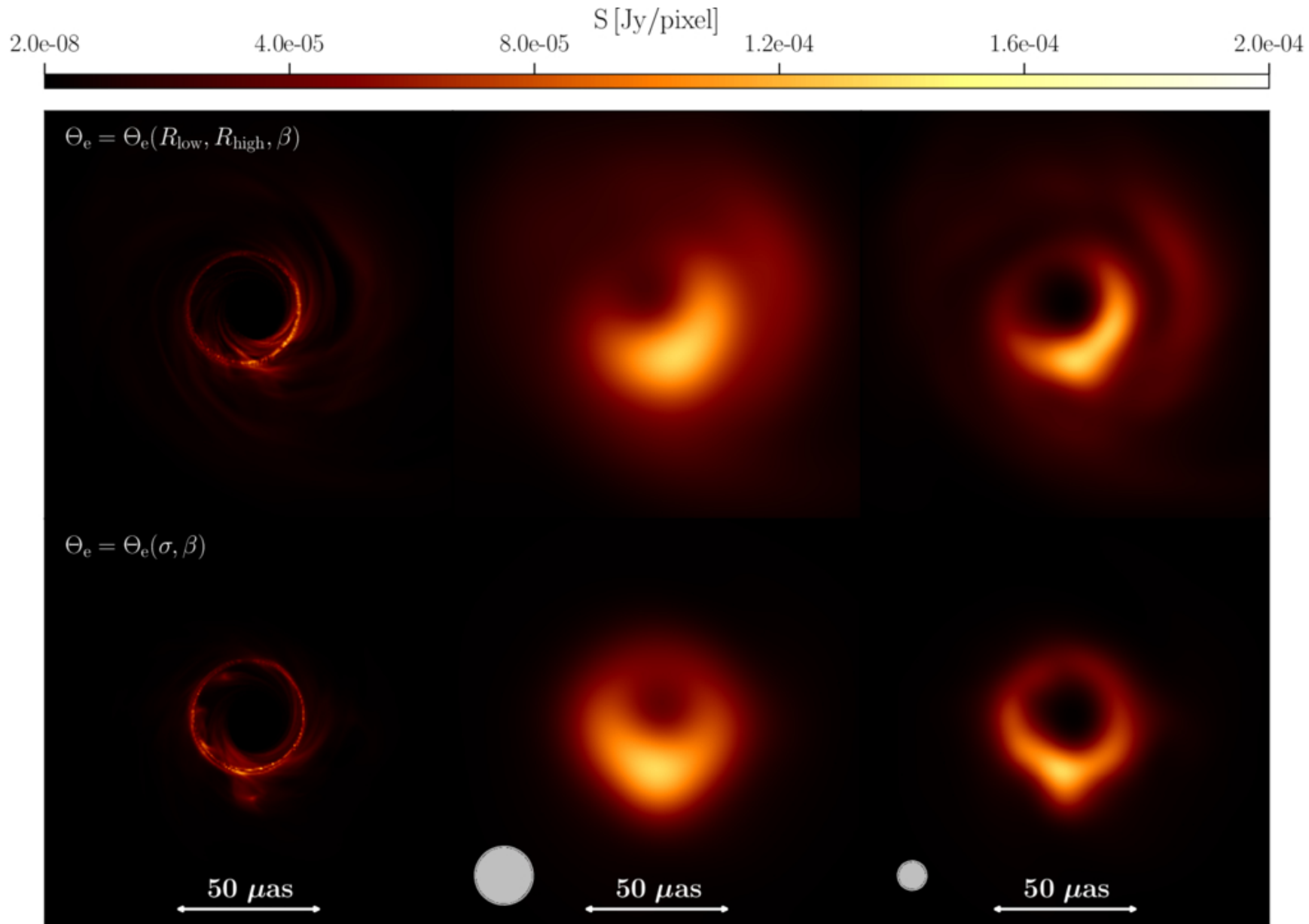
Figure 6. from Alejandro Cruz-Osorio et al 2026 Astrophys. J. 1001 doi:10.3847/1538-4357/ae4b3d https://dx.doi.org/10.3847/1538-4357/ae4b3d © 2026. The Author(s). Published by the American Astronomical Society.
