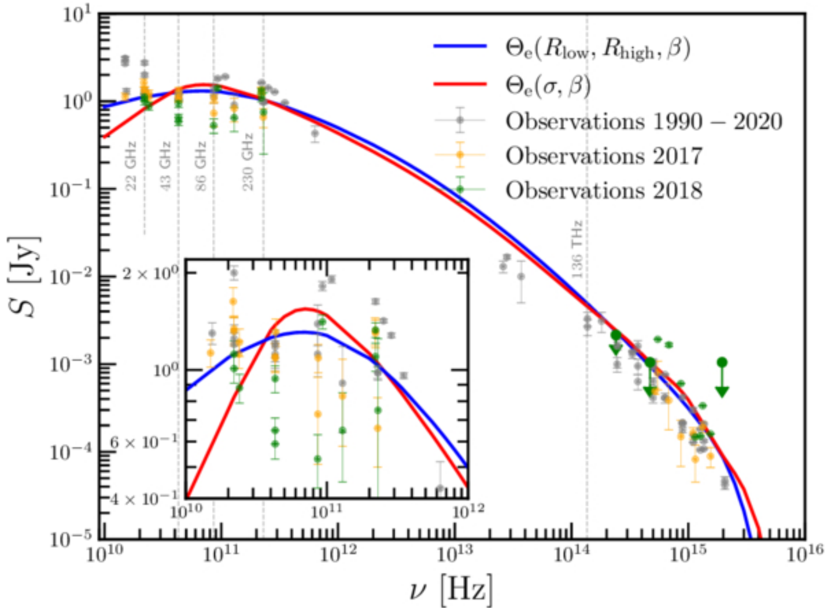
Figure 5. from Alejandro Cruz-Osorio et al 2026 Astrophys. J. 1001 doi:10.3847/1538-4357/ae4b3d https://dx.doi.org/10.3847/1538-4357/ae4b3d © 2026. The Author(s). Published by the American Astronomical Society.
