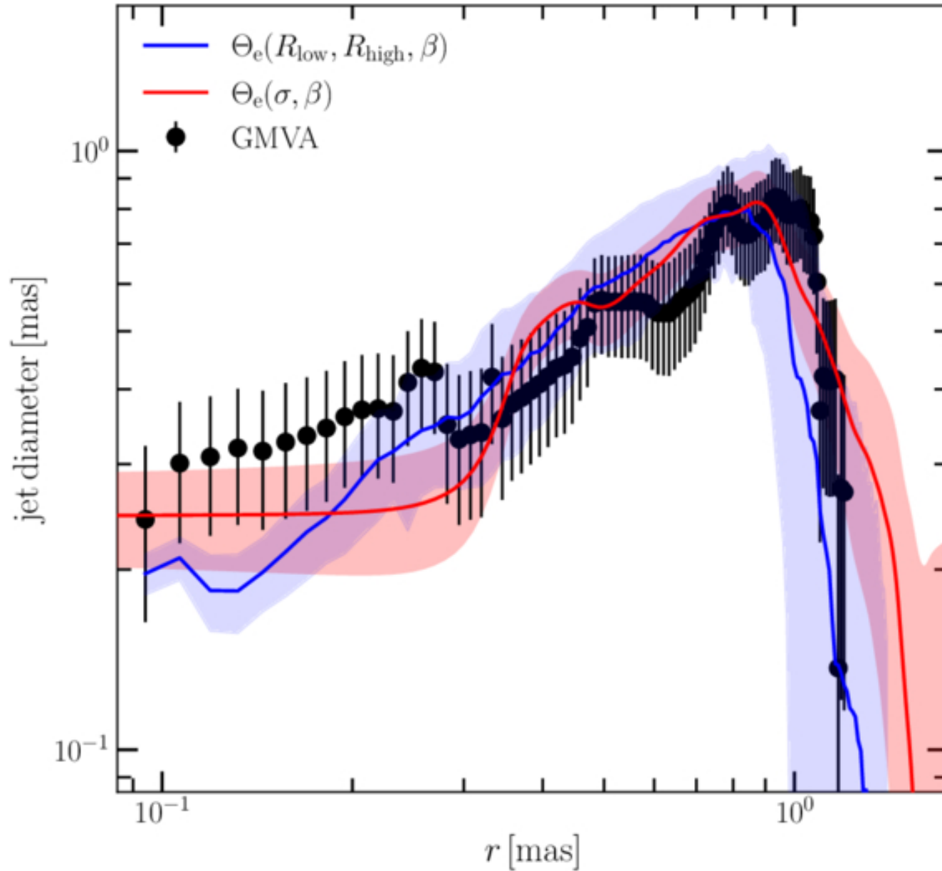
Figure 4. from Alejandro Cruz-Osorio et al 2026 Astrophys. J. 1001 doi:10.3847/1538-4357/ae4b3d https://dx.doi.org/10.3847/1538-4357/ae4b3d © 2026. The Author(s). Published by the American Astronomical Society.
