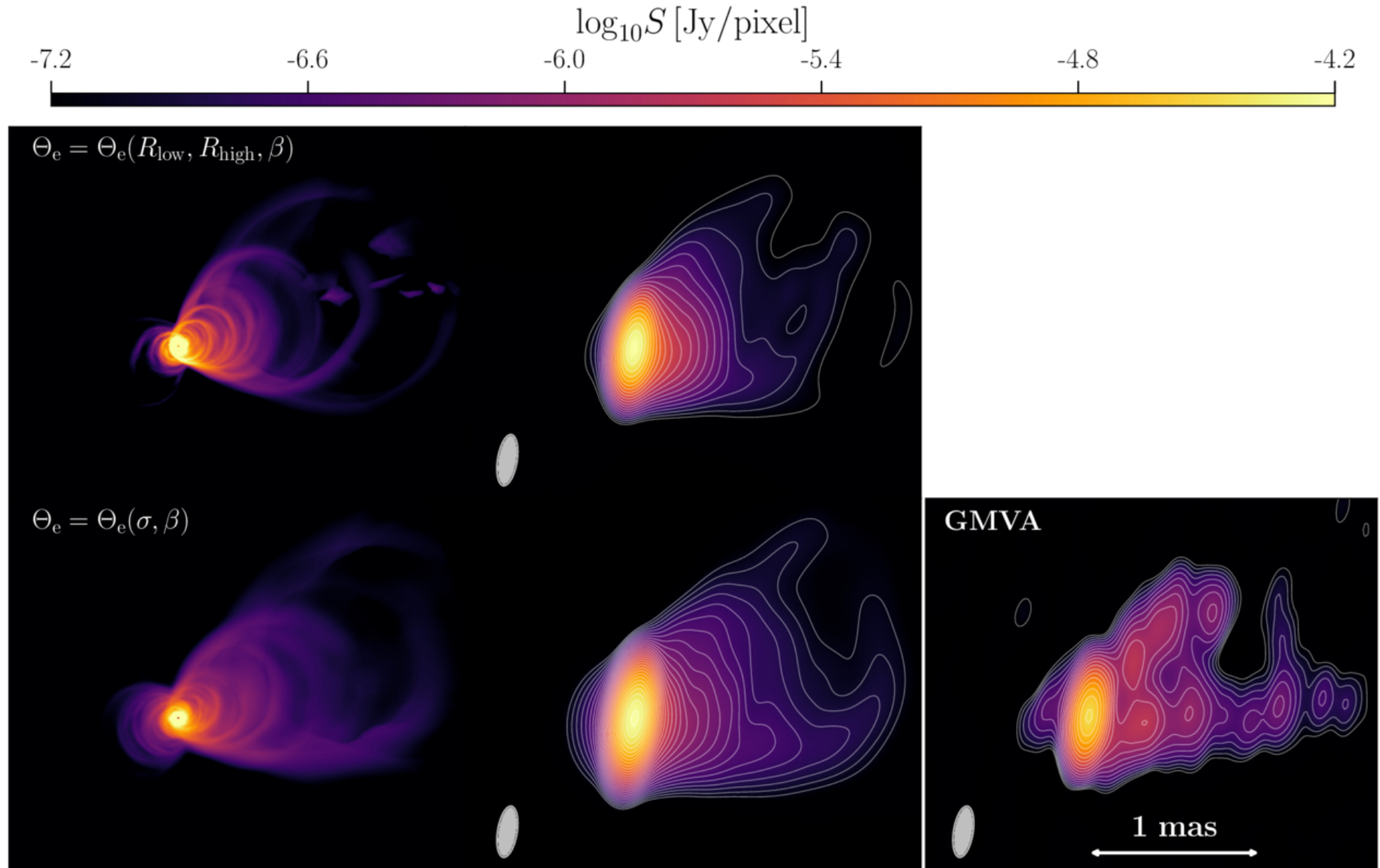
Figure 3. from Alejandro Cruz-Osorio et al 2026 Astrophys. J. 1001 doi:10.3847/1538-4357/ae4b3d https://dx.doi.org/10.3847/1538-4357/ae4b3d © 2026. The Author(s). Published by the American Astronomical Society.
