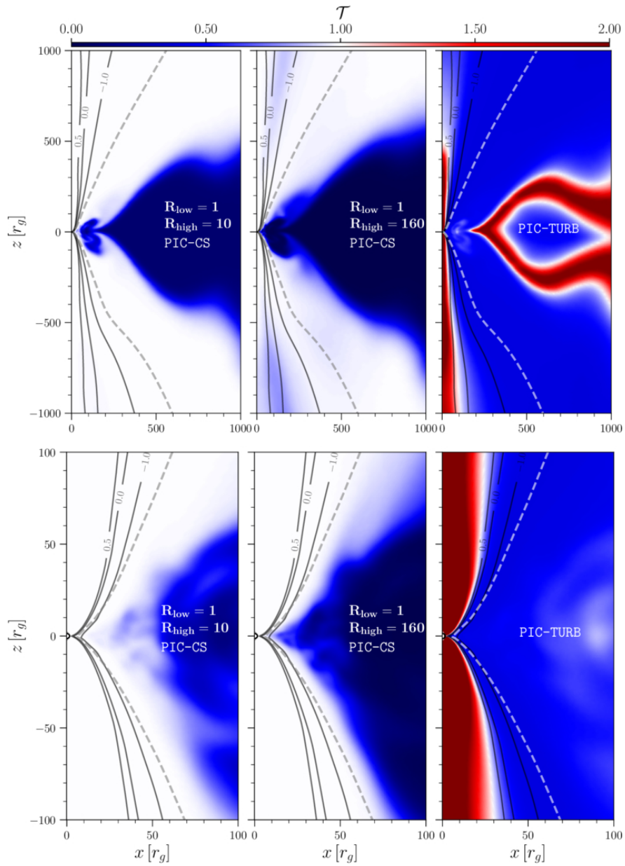
Figure 2. from Alejandro Cruz-Osorio et al 2026 Astrophys. J. 1001 doi:10.3847/1538-4357/ae4b3d https://dx.doi.org/10.3847/1538-4357/ae4b3d © 2026. The Author(s). Published by the American Astronomical Society.
