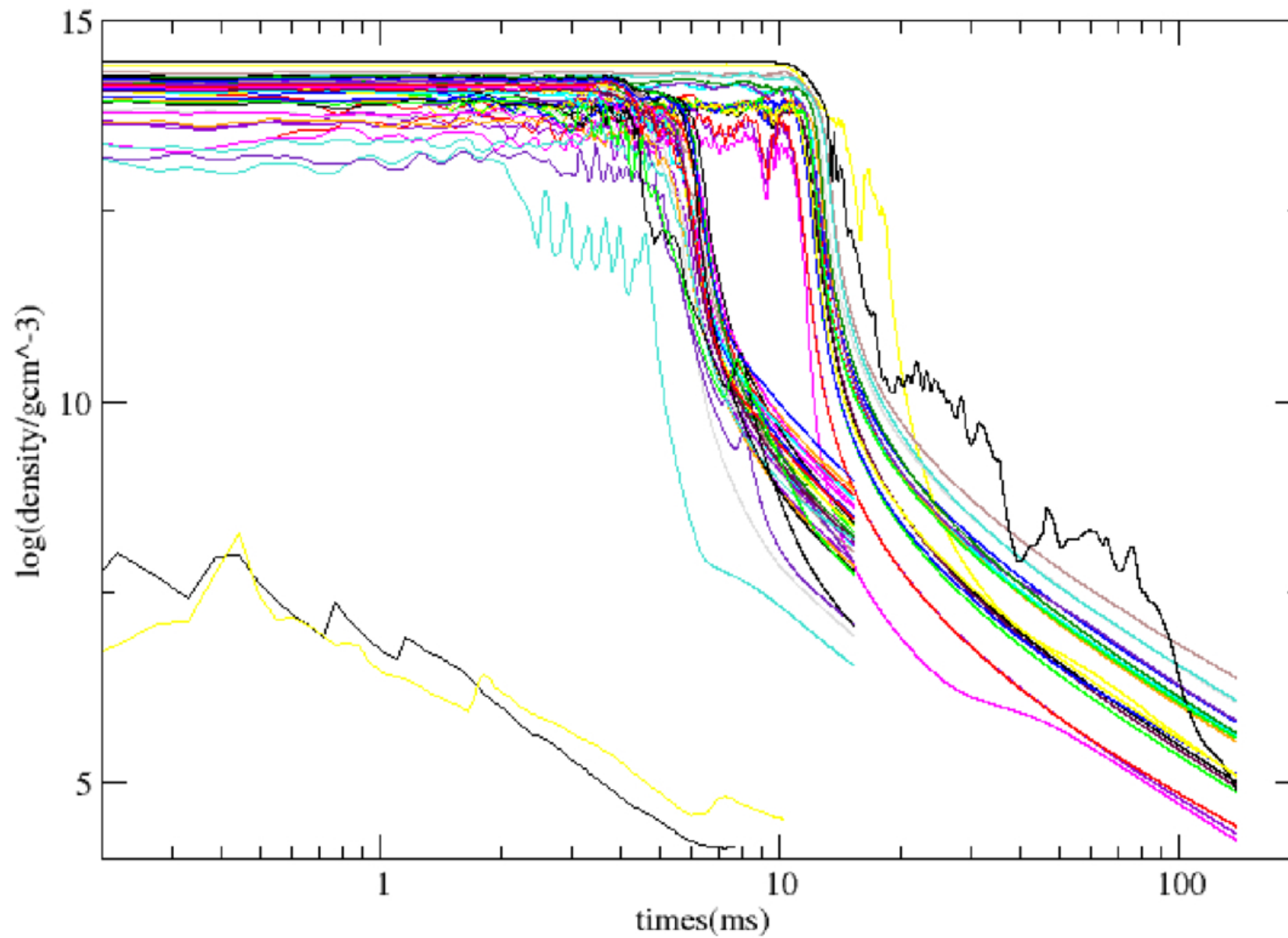
Figure 3. from Rita K. Y. Lau 2026 Astrophys. J. 1000 doi:10.3847/1538-4357/ae4b31 https://dx.doi.org/10.3847/1538-4357/ae4b31 © 2026. The Author(s). Published by the American Astronomical Society.
