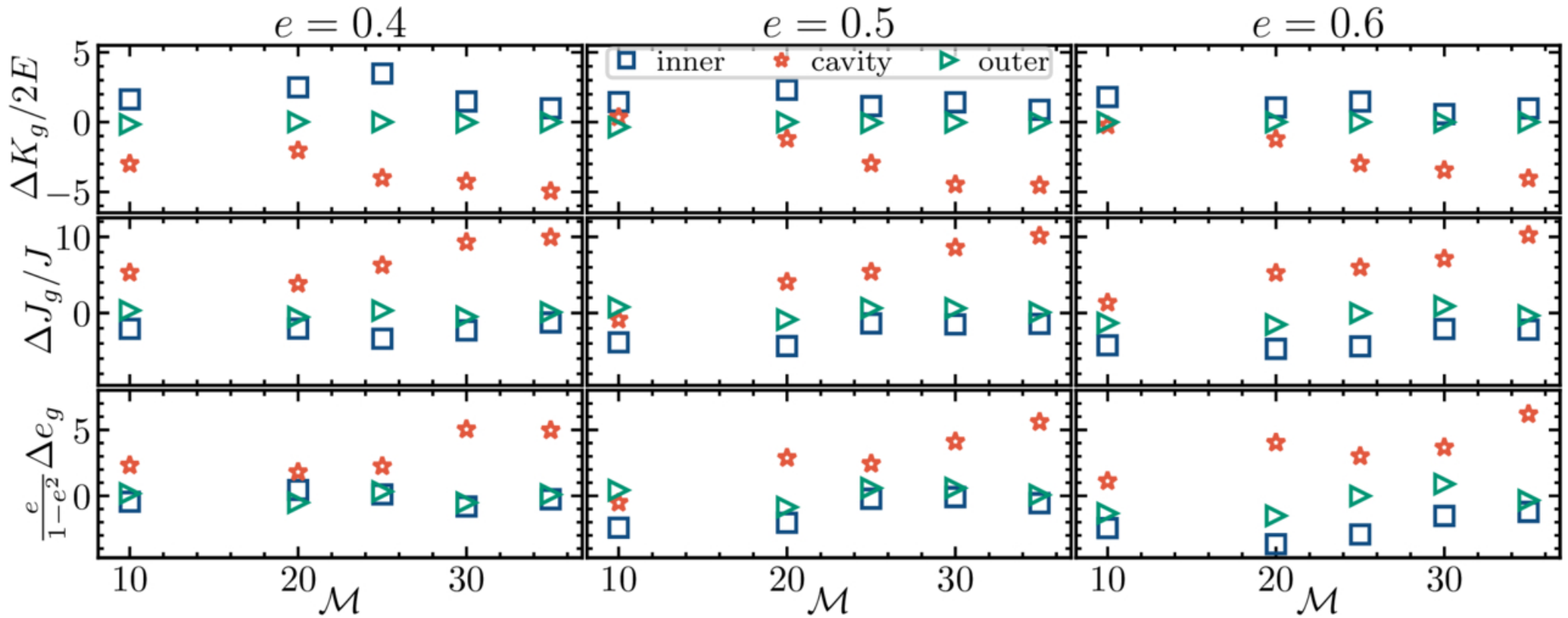
Figure 9. from Alexander J. Dittmann et al 2026 Astrophys. J. 1001 doi:10.3847/1538-4357/ae4a9c https://dx.doi.org/10.3847/1538-4357/ae4a9c © 2026. The Author(s). Published by the American Astronomical Society.
