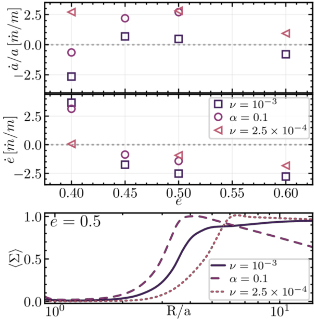
Figure 7. from Alexander J. Dittmann et al 2026 Astrophys. J. 1001 doi:10.3847/1538-4357/ae4a9c https://dx.doi.org/10.3847/1538-4357/ae4a9c © 2026. The Author(s). Published by the American Astronomical Society.
