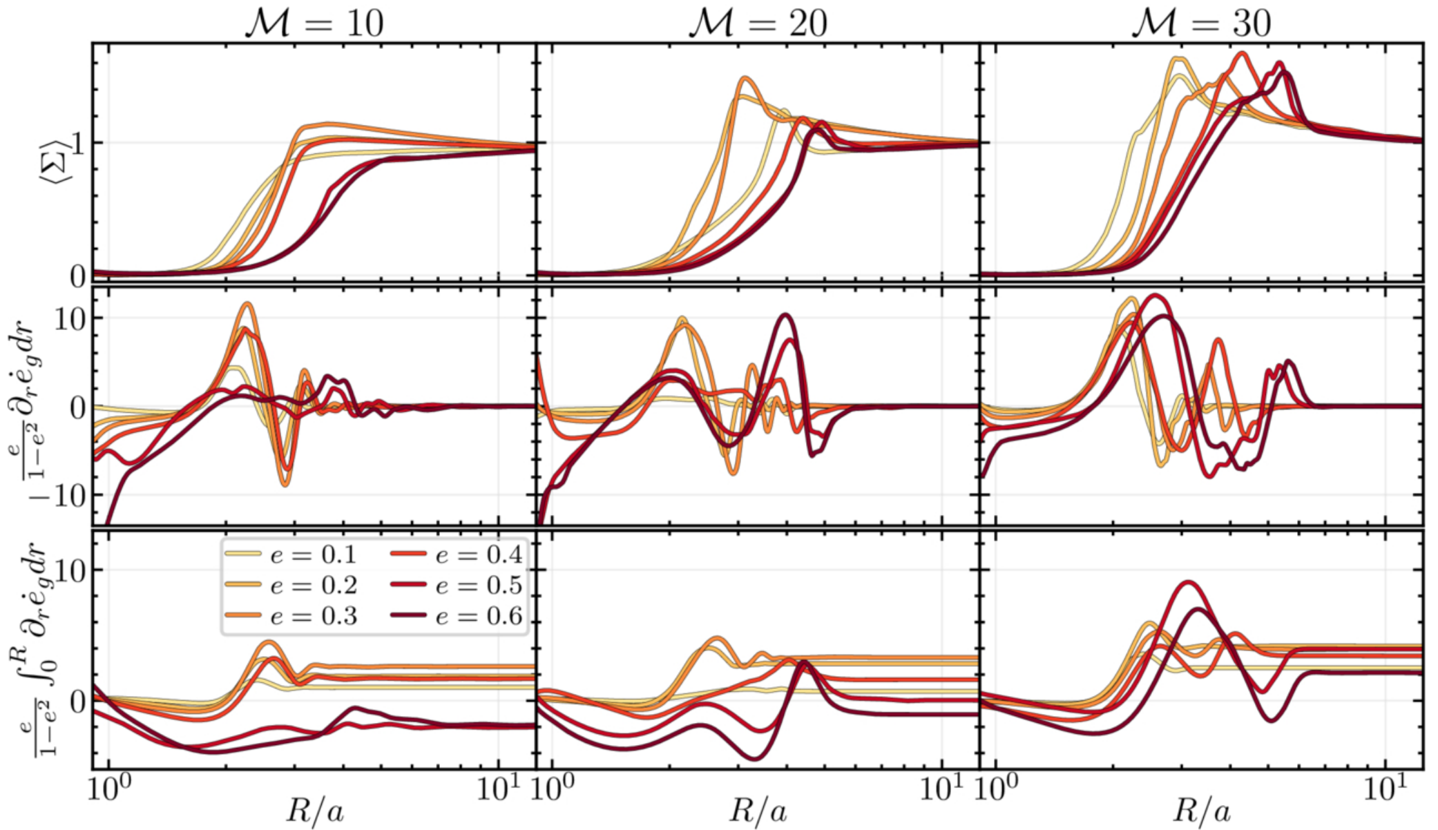
Figure 6. from Alexander J. Dittmann et al 2026 Astrophys. J. 1001 doi:10.3847/1538-4357/ae4a9c https://dx.doi.org/10.3847/1538-4357/ae4a9c © 2026. The Author(s). Published by the American Astronomical Society.
