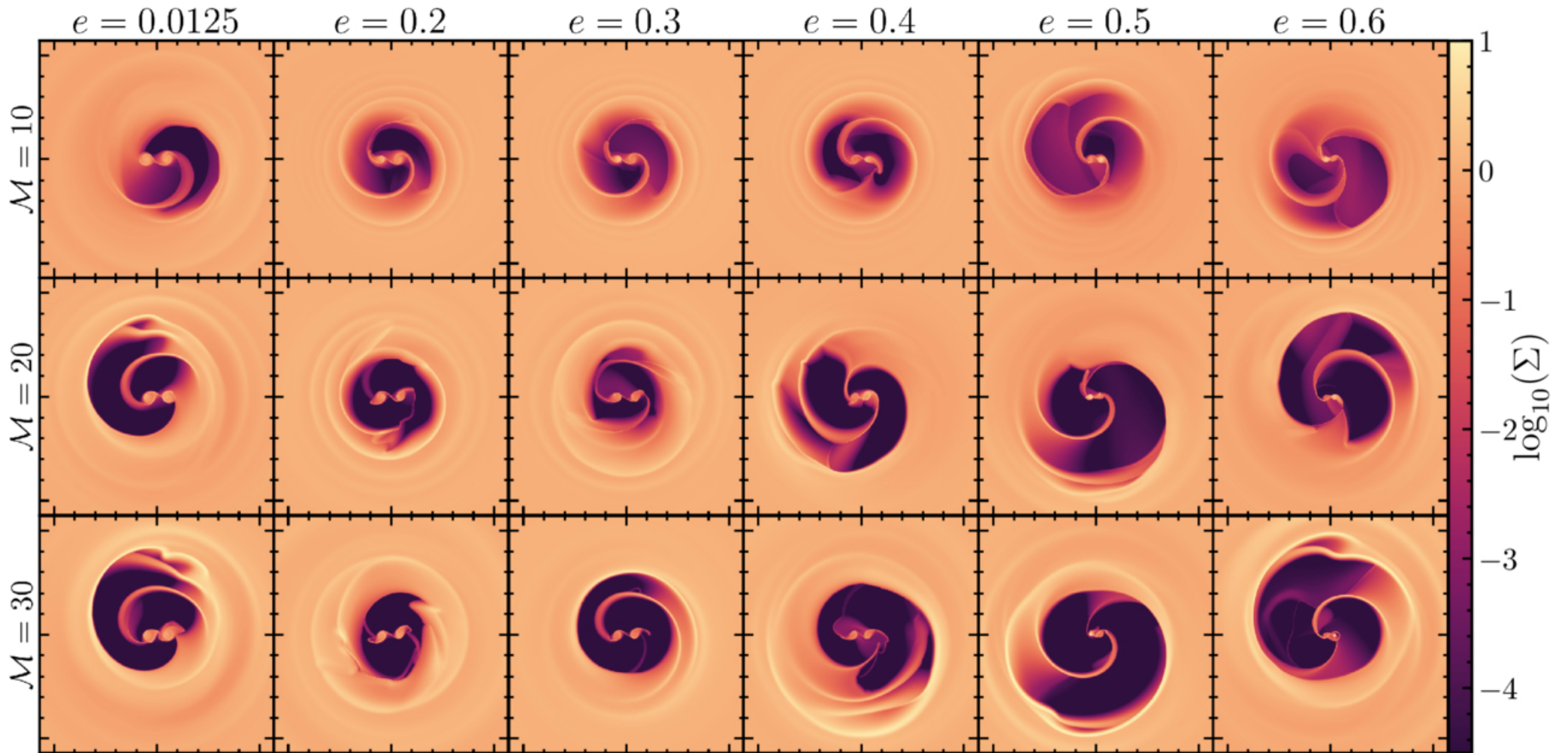
Figure 2. from Alexander J. Dittmann et al 2026 Astrophys. J. 1001 doi:10.3847/1538-4357/ae4a9c https://dx.doi.org/10.3847/1538-4357/ae4a9c © 2026. The Author(s). Published by the American Astronomical Society.
