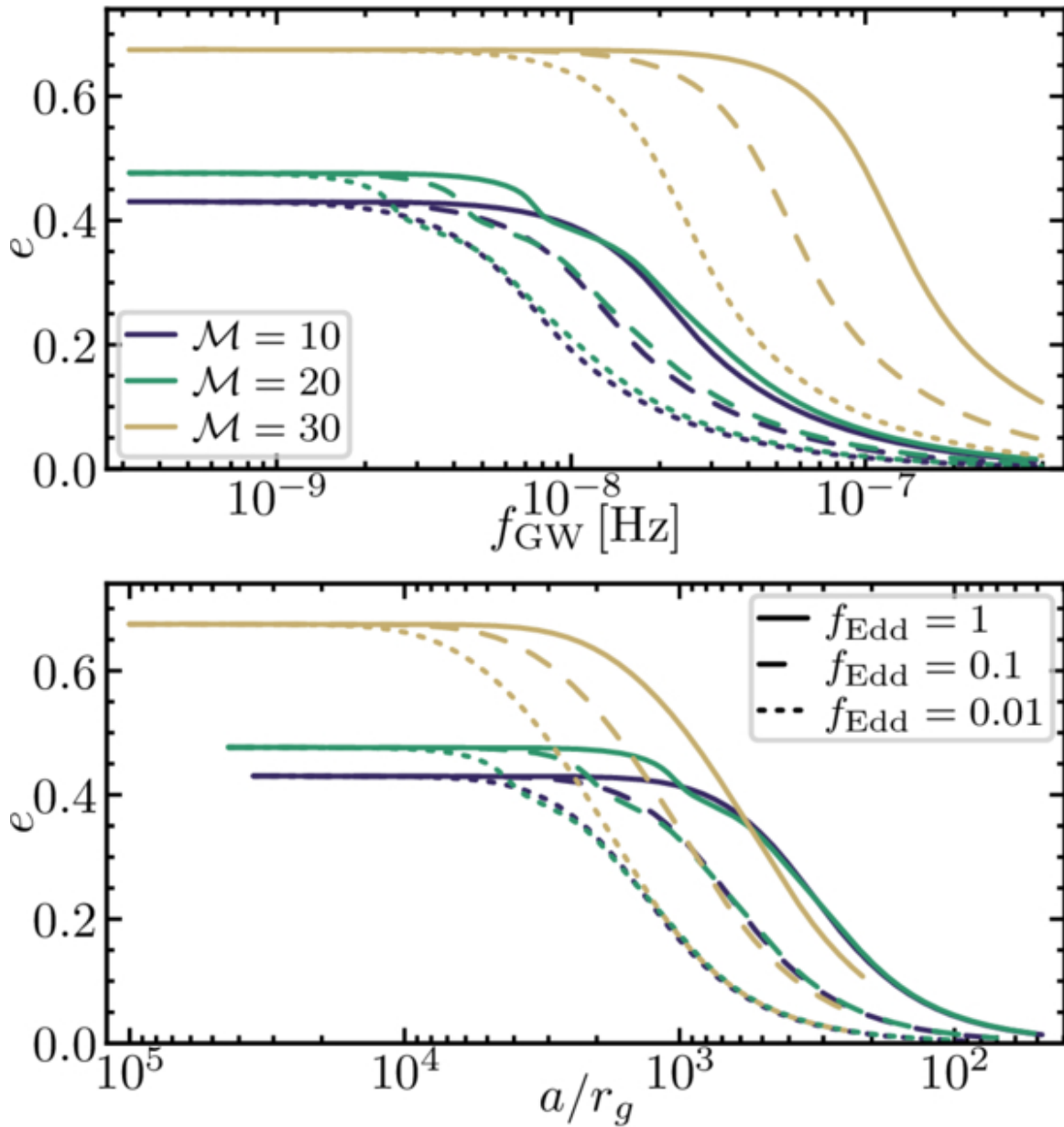
Figure 12. from Alexander J. Dittmann et al 2026 Astrophys. J. 1001 doi:10.3847/1538-4357/ae4a9c https://dx.doi.org/10.3847/1538-4357/ae4a9c © 2026. The Author(s). Published by the American Astronomical Society.
