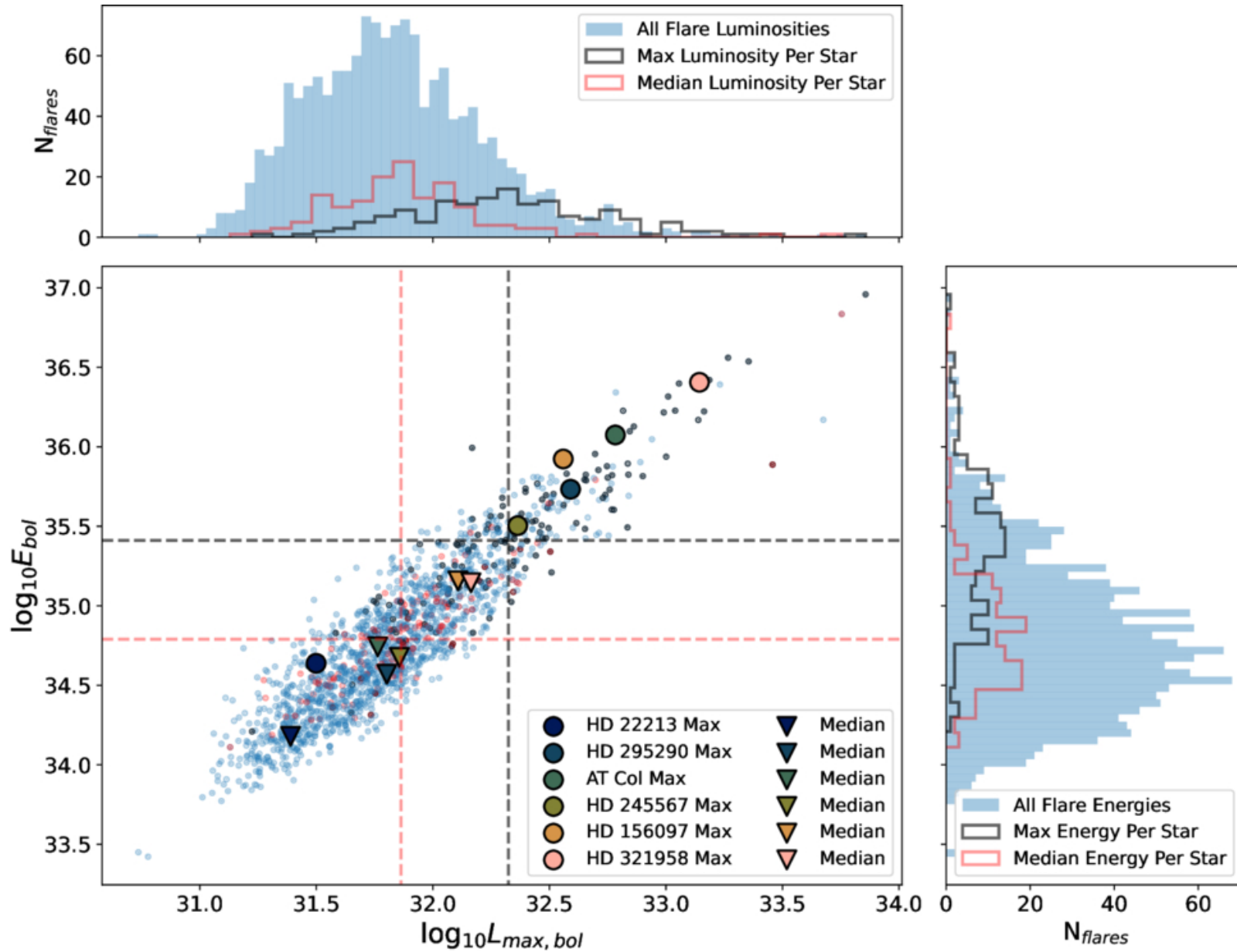
Figure 5. from Ivey Davis et al 2026 Astrophys. J. 1001 doi:10.3847/1538-4357/ae4a22 https://dx.doi.org/10.3847/1538-4357/ae4a22 © 2026. The Author(s). Published by the American Astronomical Society.
