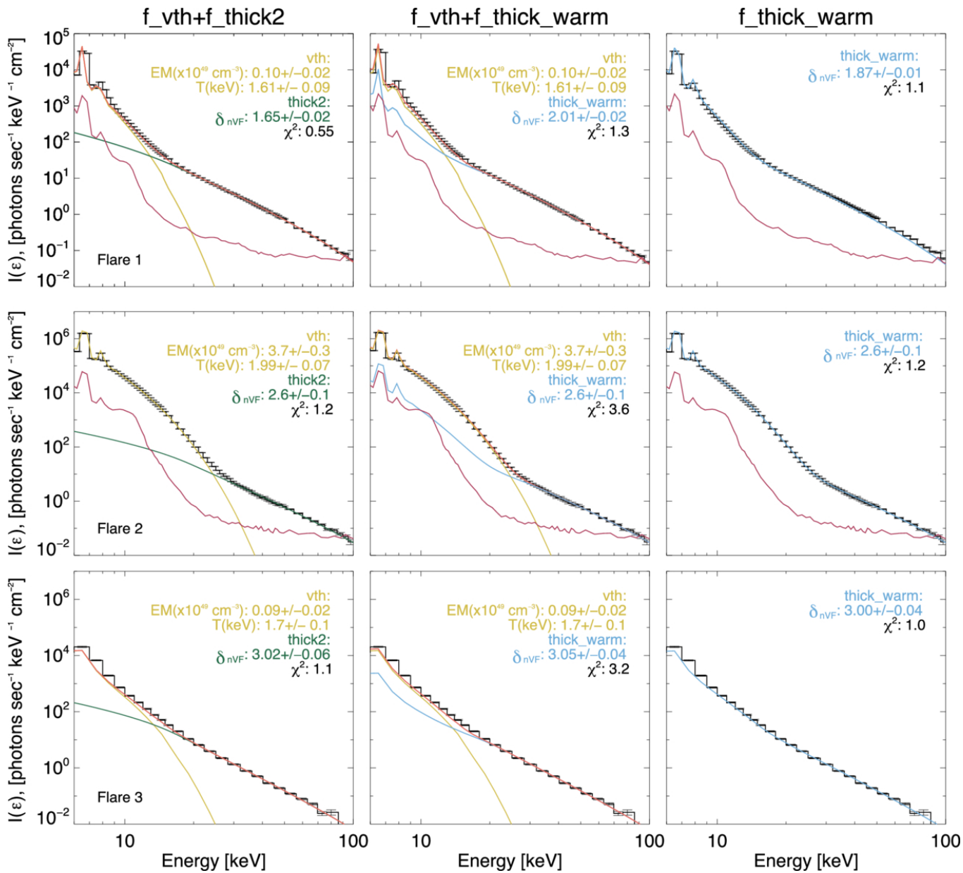
Figure 7. from Morgan Stores et al 2026 Astrophys. J. 1001 doi:10.3847/1538-4357/ae47d7 https://dx.doi.org/10.3847/1538-4357/ae47d7 © 2026. The Author(s). Published by the American Astronomical Society.
