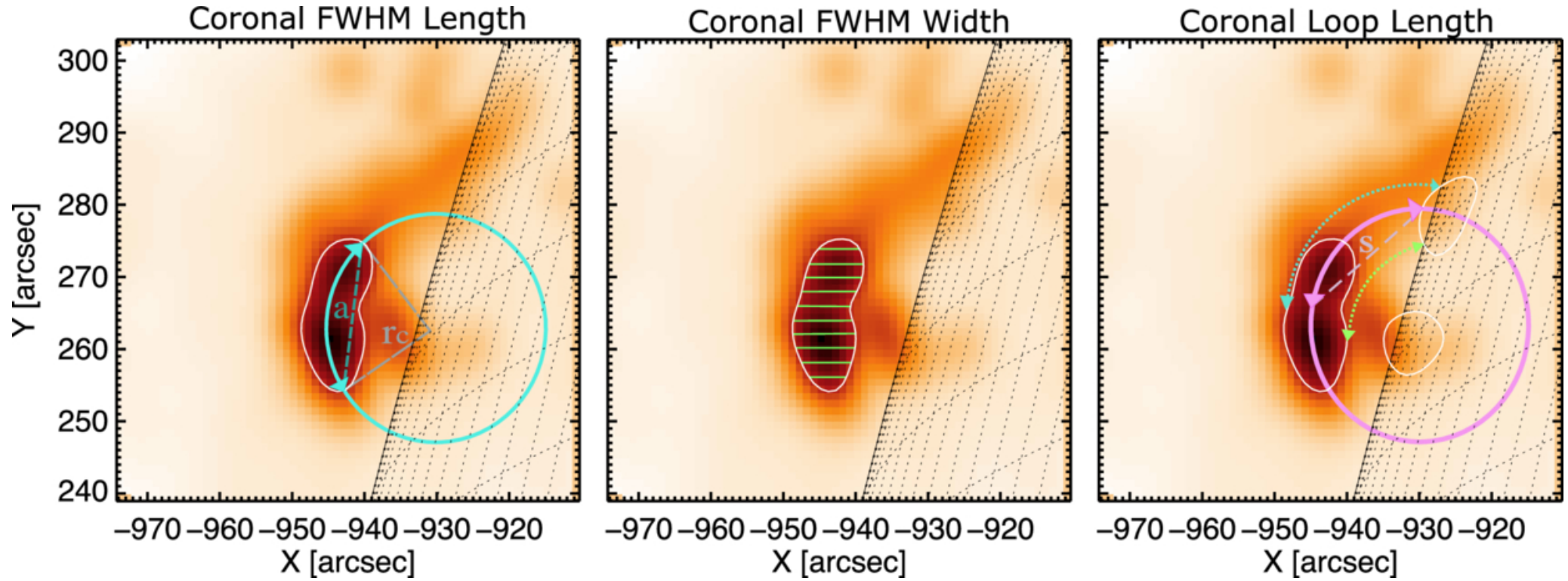
Figure 6. from Morgan Stores et al 2026 Astrophys. J. 1001 doi:10.3847/1538-4357/ae47d7 https://dx.doi.org/10.3847/1538-4357/ae47d7 © 2026. The Author(s). Published by the American Astronomical Society.
