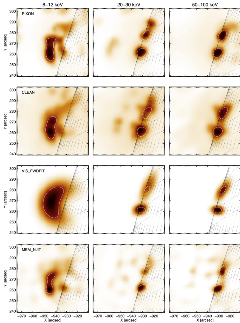
Figure 3. from Morgan Stores et al 2026 Astrophys. J. 1001 doi:10.3847/1538-4357/ae47d7 https://dx.doi.org/10.3847/1538-4357/ae47d7 © 2026. The Author(s). Published by the American Astronomical Society.
