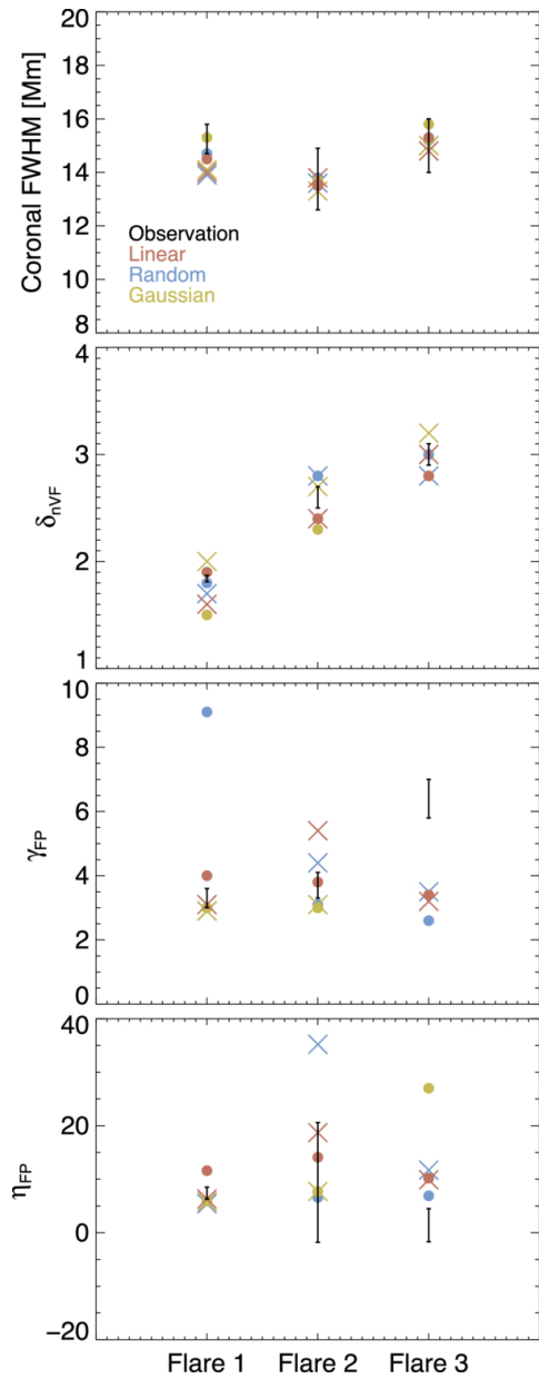
Figure 12. from Morgan Stores et al 2026 Astrophys. J. 1001 doi:10.3847/1538-4357/ae47d7 https://dx.doi.org/10.3847/1538-4357/ae47d7 © 2026. The Author(s). Published by the American Astronomical Society.
