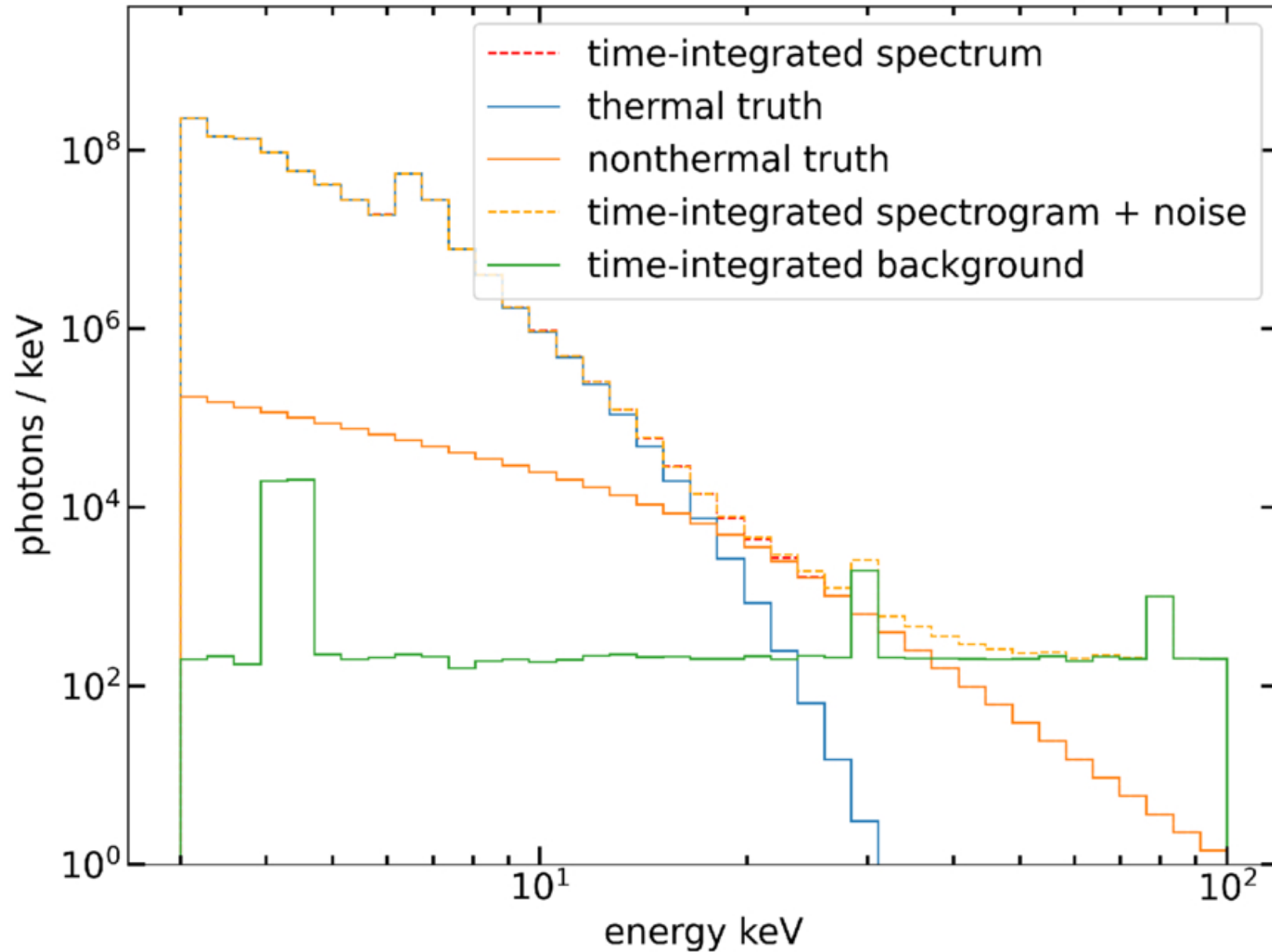
Figure 9. from William Setterberg and Lindsay Glesener 2026 Astrophys. J. 1000 doi:10.3847/1538-4357/ae462b https://dx.doi.org/10.3847/1538-4357/ae462b © 2026. The Author(s). Published by the American Astronomical Society.
