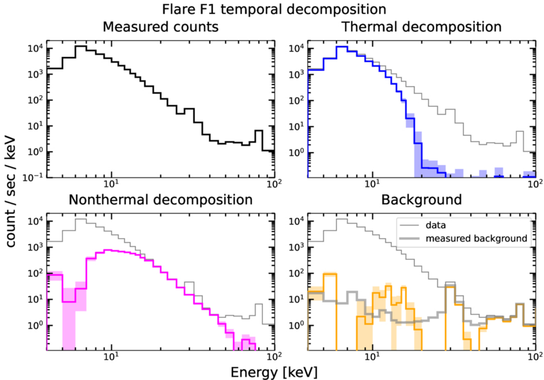
Figure 2. from William Setterberg and Lindsay Glesener 2026 Astrophys. J. 1000 doi:10.3847/1538-4357/ae462b https://dx.doi.org/10.3847/1538-4357/ae462b © 2026. The Author(s). Published by the American Astronomical Society.
