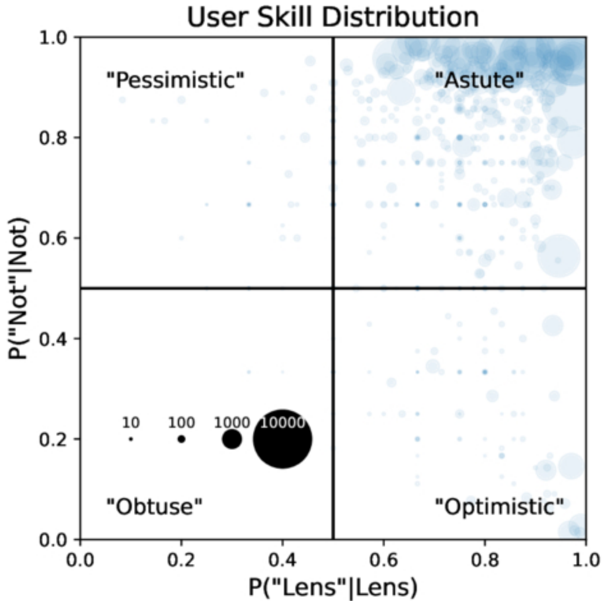
Figure 9. from J. González et al 2026 Astrophys. J. 1002 doi:10.3847/1538-4357/ae450c https://dx.doi.org/10.3847/1538-4357/ae450c © 2026. The Author(s). Published by the American Astronomical Society.
