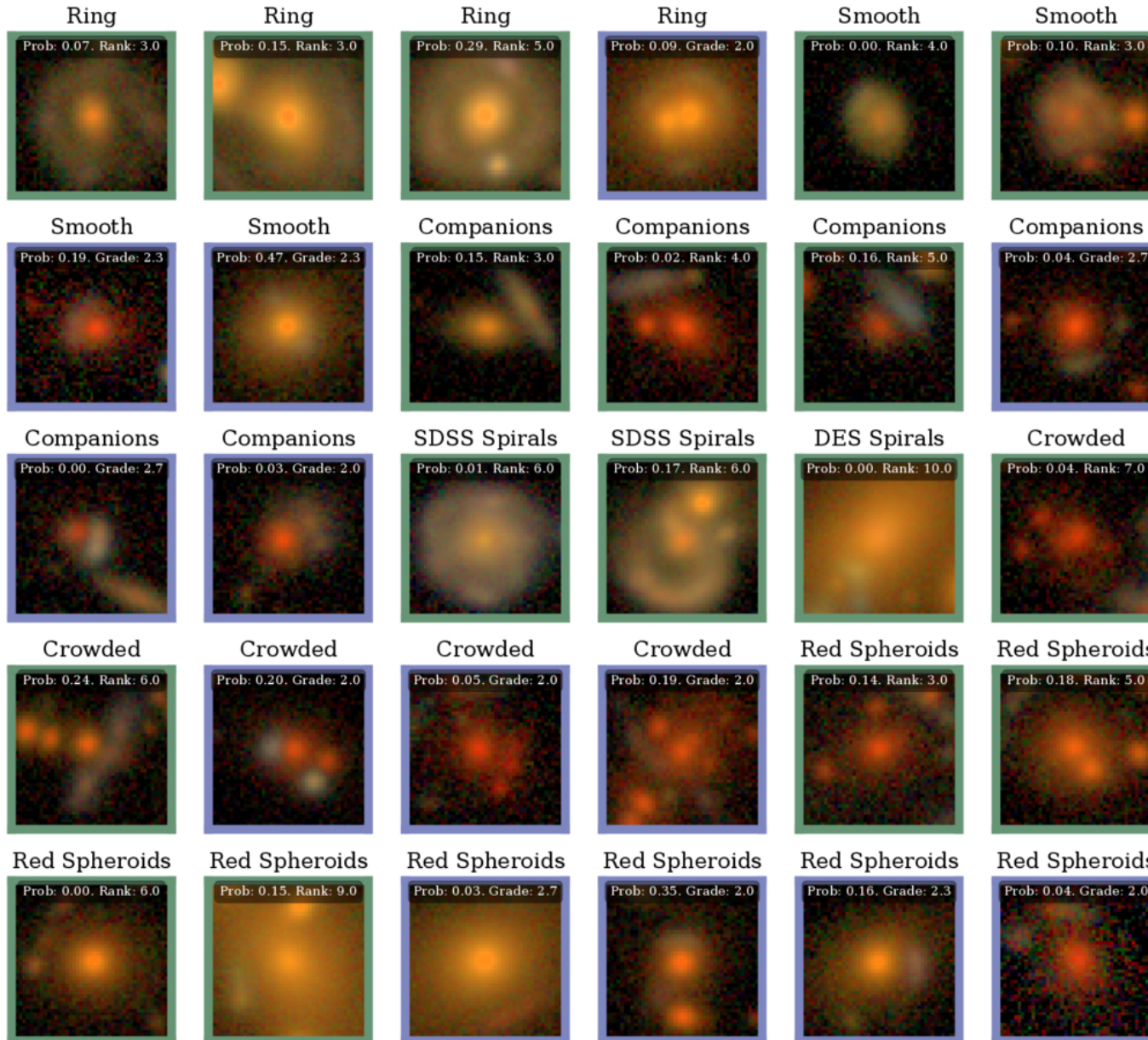
Figure 6. from J. González et al 2026 Astrophys. J. 1002 doi:10.3847/1538-4357/ae450c https://dx.doi.org/10.3847/1538-4357/ae450c © 2026. The Author(s). Published by the American Astronomical Society.
