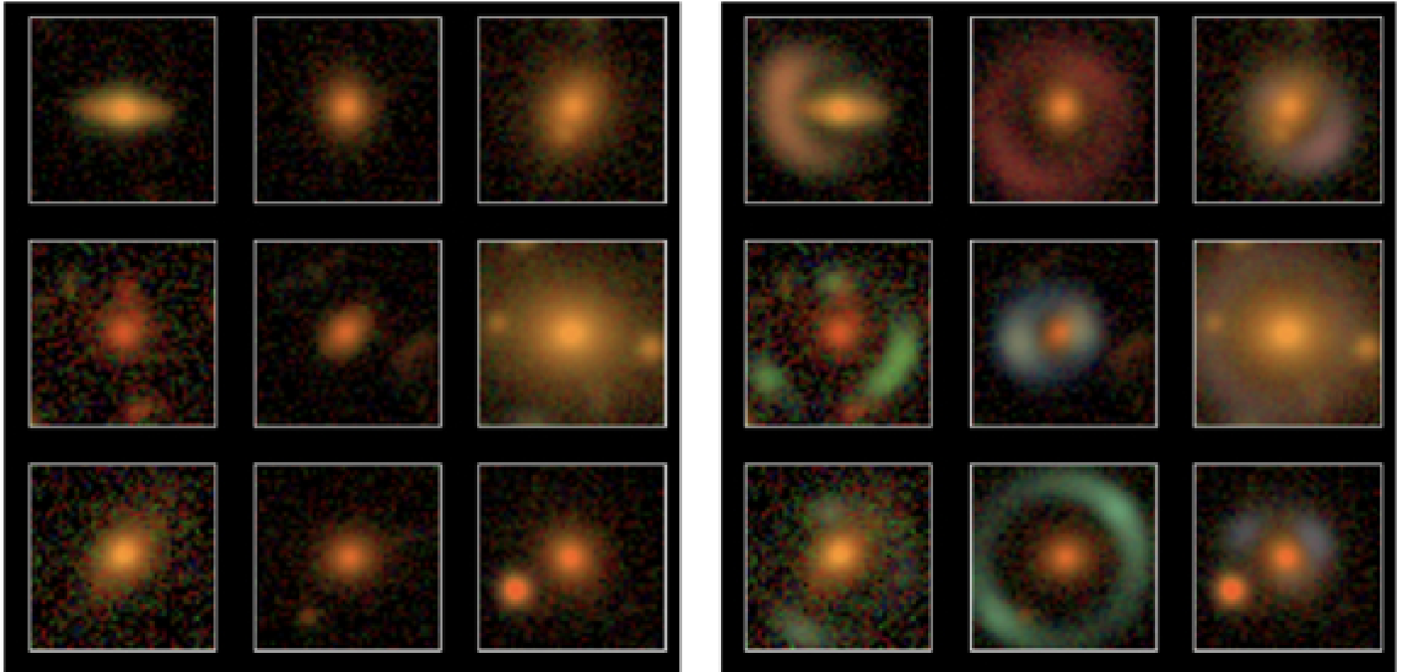
Figure 2. from J. González et al 2026 Astrophys. J. 1002 doi:10.3847/1538-4357/ae450c https://dx.doi.org/10.3847/1538-4357/ae450c © 2026. The Author(s). Published by the American Astronomical Society.
