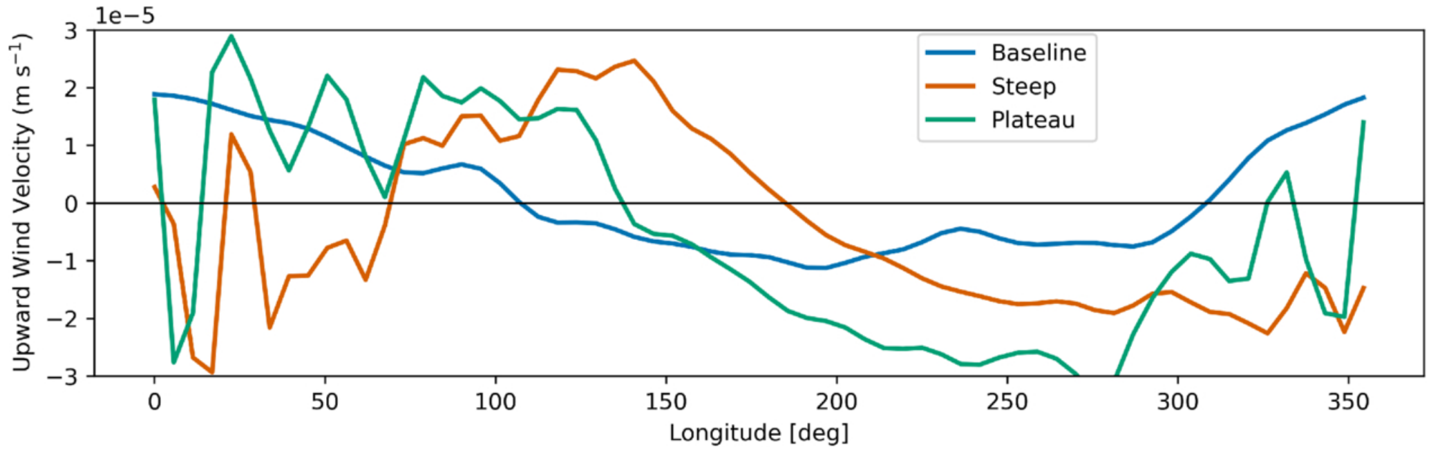
Figure 9. from Howard Chen et al 2026 Astrophys. J. 1001 doi:10.3847/1538-4357/ae4485 https://dx.doi.org/10.3847/1538-4357/ae4485 © 2026. The Author(s). Published by the American Astronomical Society.
