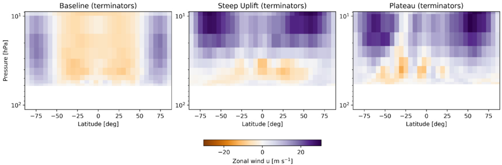
Figure 7. from Howard Chen et al 2026 Astrophys. J. 1001 doi:10.3847/1538-4357/ae4485 https://dx.doi.org/10.3847/1538-4357/ae4485 © 2026. The Author(s). Published by the American Astronomical Society.
