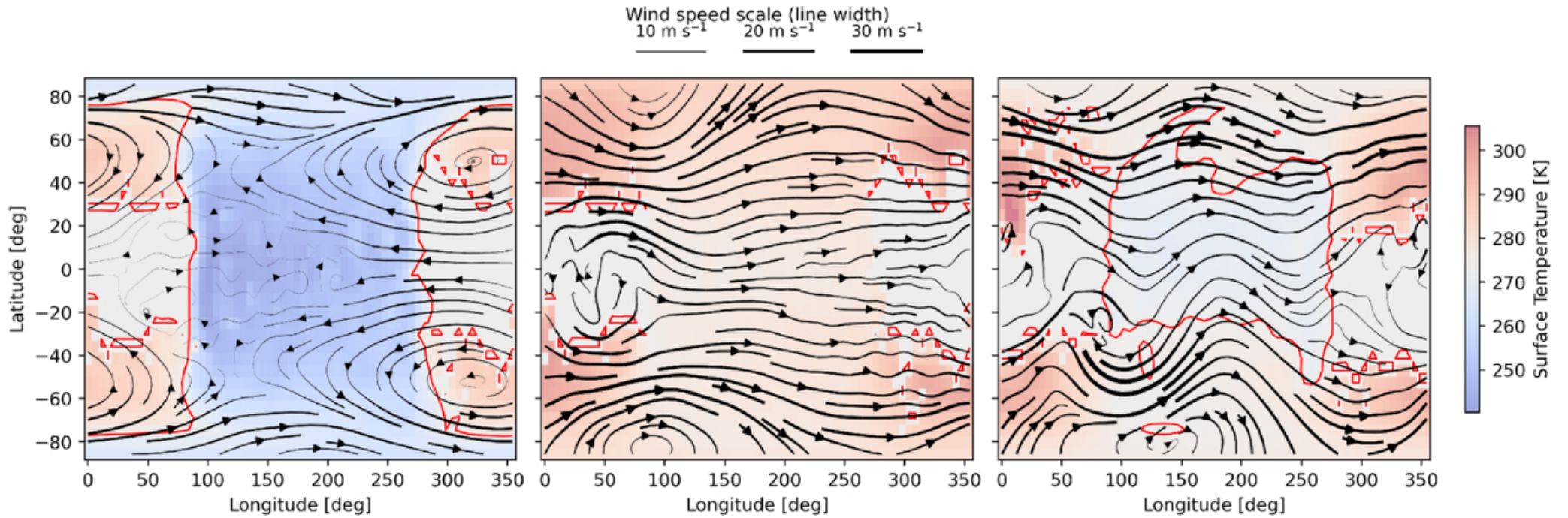
Figure 6. from Howard Chen et al 2026 Astrophys. J. 1001 doi:10.3847/1538-4357/ae4485 https://dx.doi.org/10.3847/1538-4357/ae4485 © 2026. The Author(s). Published by the American Astronomical Society.
