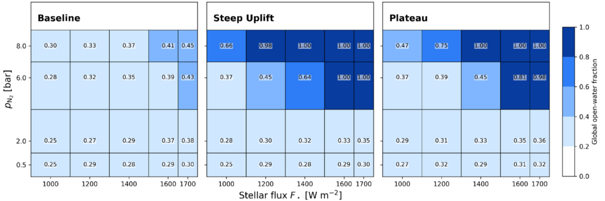
Figure 2. from Howard Chen et al 2026 Astrophys. J. 1001 doi:10.3847/1538-4357/ae4485 https://dx.doi.org/10.3847/1538-4357/ae4485 © 2026. The Author(s). Published by the American Astronomical Society.
