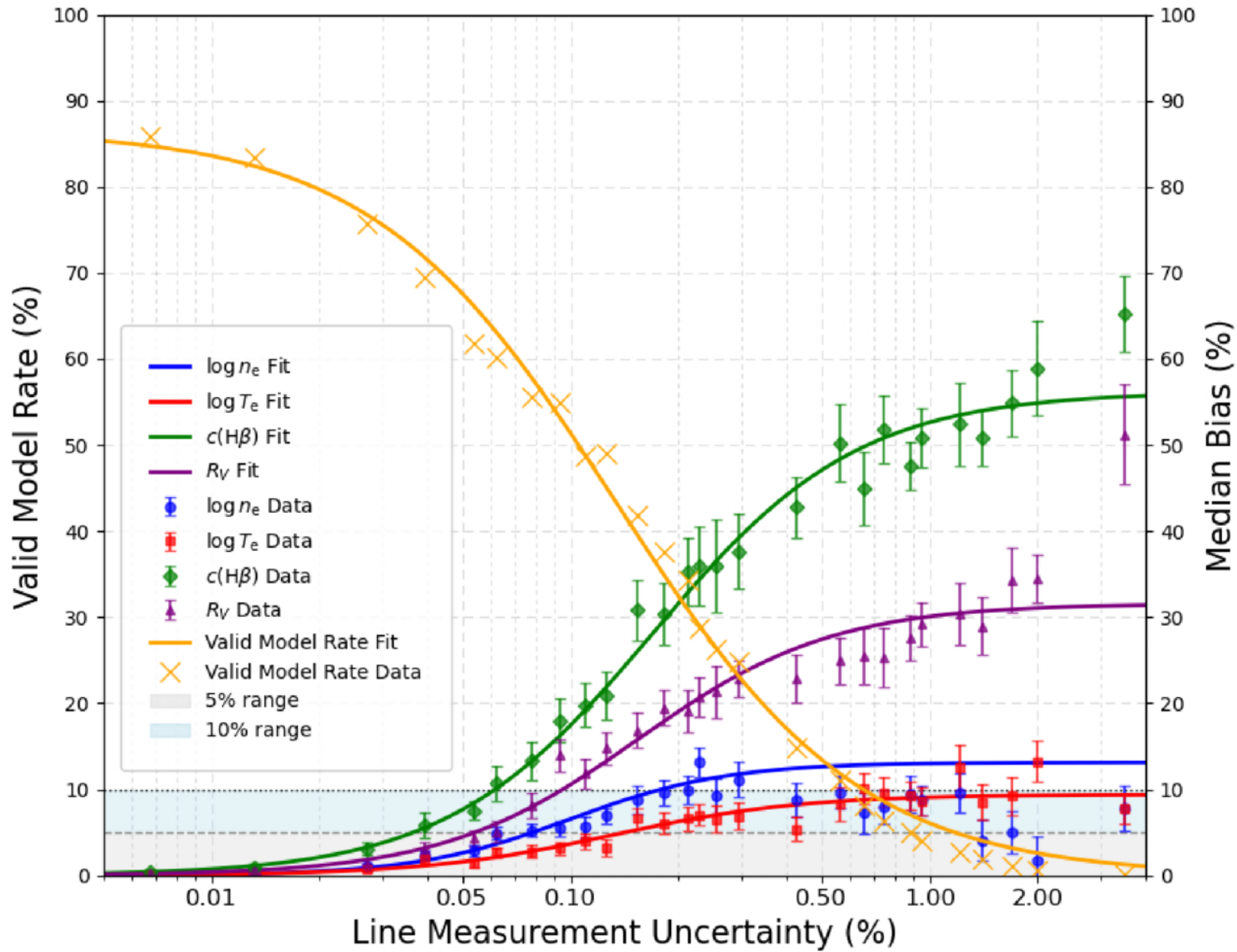
Figure 2. from Toshiya Ueta et al 2026 Astrophys. J. 999 doi:10.3847/1538-4357/ae4347 https://dx.doi.org/10.3847/1538-4357/ae4347 © 2026. The Author(s). Published by the American Astronomical Society.
