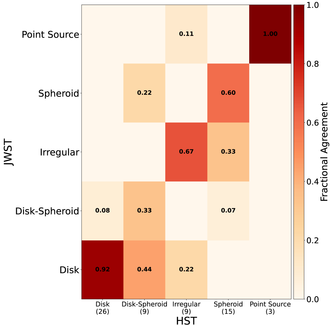
Figure 9. from William W.H. Jarvis et al 2026 Astrophys. J. 1001 doi:10.3847/1538-4357/ae40b4 https://dx.doi.org/10.3847/1538-4357/ae40b4 © 2026. The Author(s). Published by the American Astronomical Society.
