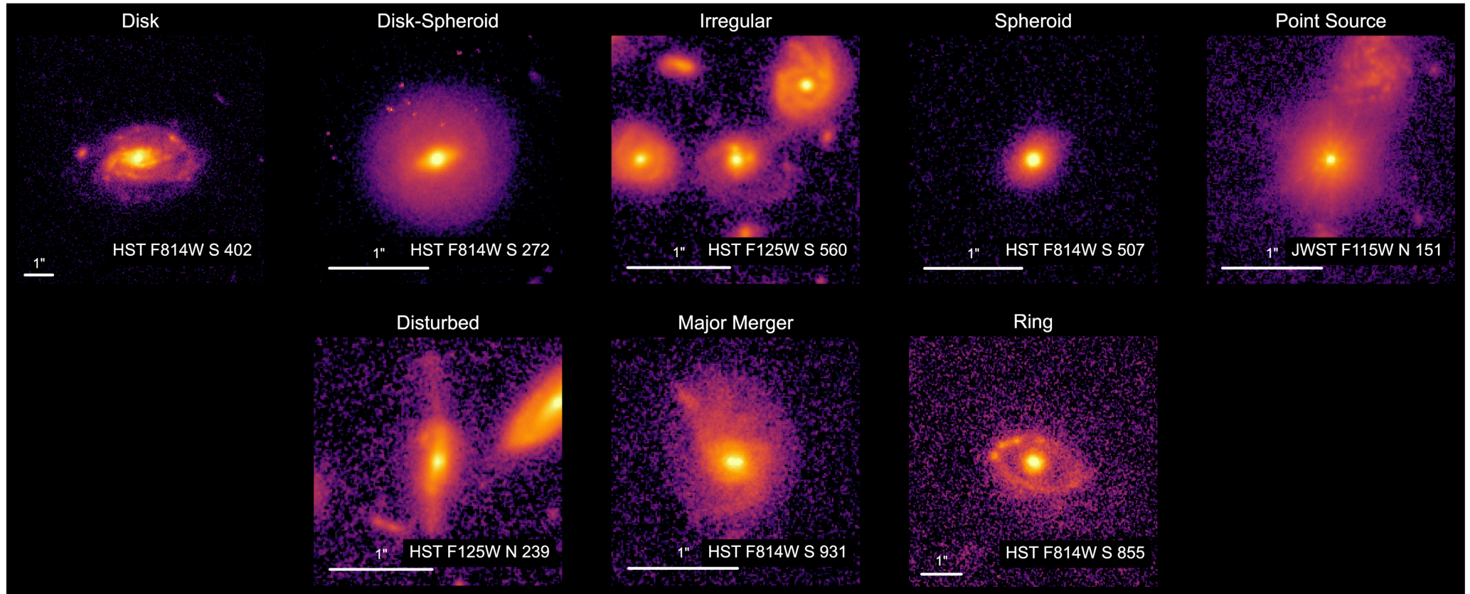
Figure 8. from William W.H. Jarvis et al 2026 Astrophys. J. 1001 doi:10.3847/1538-4357/ae40b4 https://dx.doi.org/10.3847/1538-4357/ae40b4 © 2026. The Author(s). Published by the American Astronomical Society.
