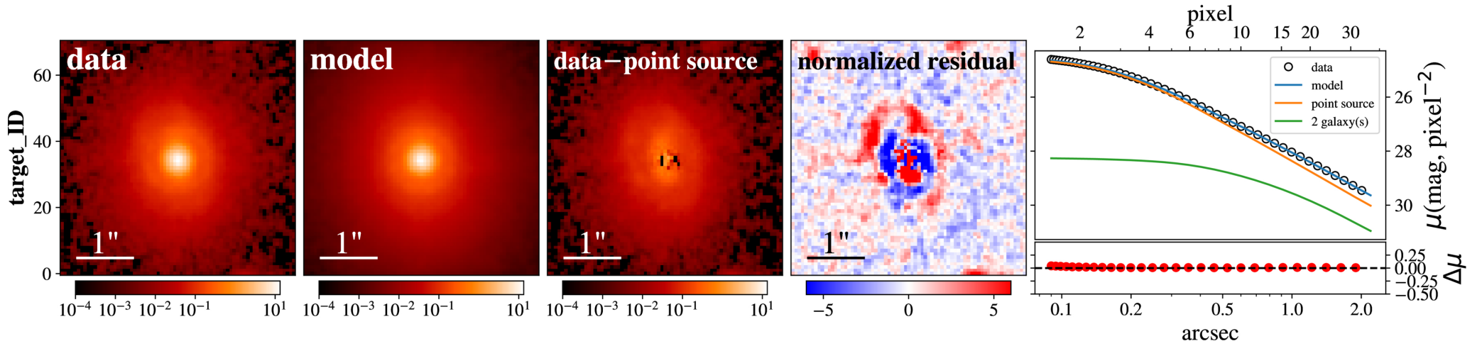
Figure 6. from William W.H. Jarvis et al 2026 Astrophys. J. 1001 doi:10.3847/1538-4357/ae40b4 https://dx.doi.org/10.3847/1538-4357/ae40b4 © 2026. The Author(s). Published by the American Astronomical Society.
