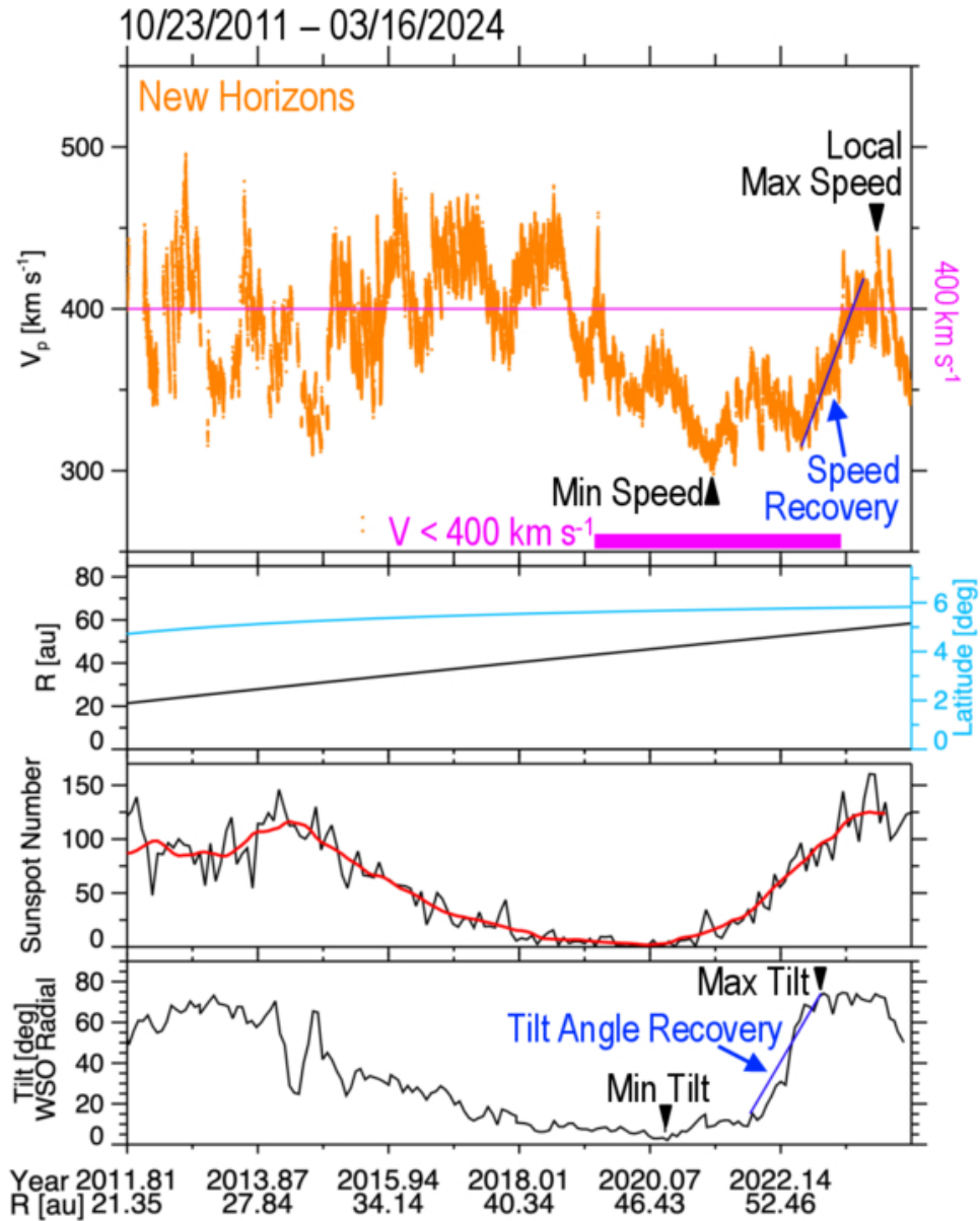
Figure 7. from Heather A. Elliott et al 2026 Astrophys. J. 1001 doi:10.3847/1538-4357/ae39c6 https://dx.doi.org/10.3847/1538-4357/ae39c6 © 2026. The Author(s). Published by the American Astronomical Society.
