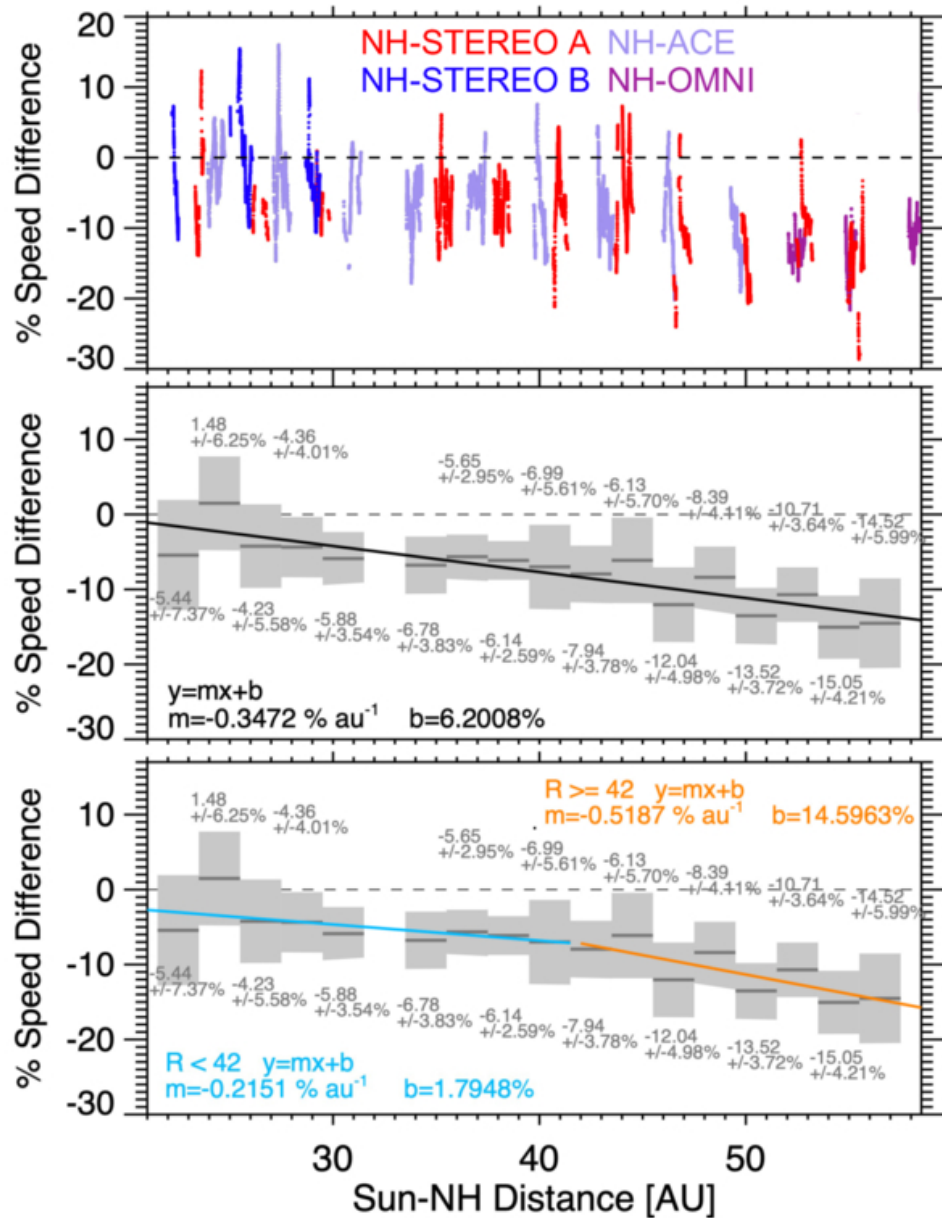
Figure 6. from Heather A. Elliott et al 2026 Astrophys. J. 1001 doi:10.3847/1538-4357/ae39c6 https://dx.doi.org/10.3847/1538-4357/ae39c6 © 2026. The Author(s). Published by the American Astronomical Society.
