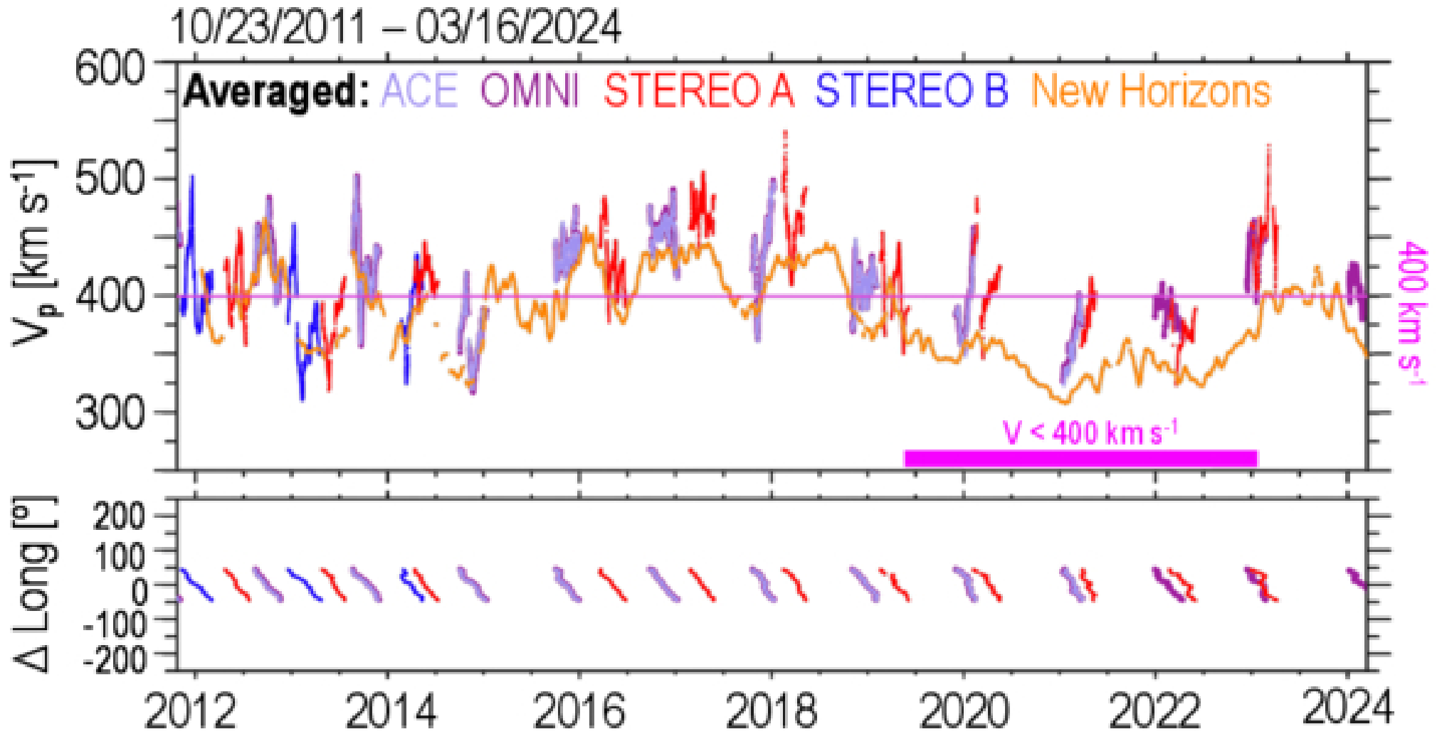
Figure 5. from Heather A. Elliott et al 2026 Astrophys. J. 1001 doi:10.3847/1538-4357/ae39c6 https://dx.doi.org/10.3847/1538-4357/ae39c6 © 2026. The Author(s). Published by the American Astronomical Society.
