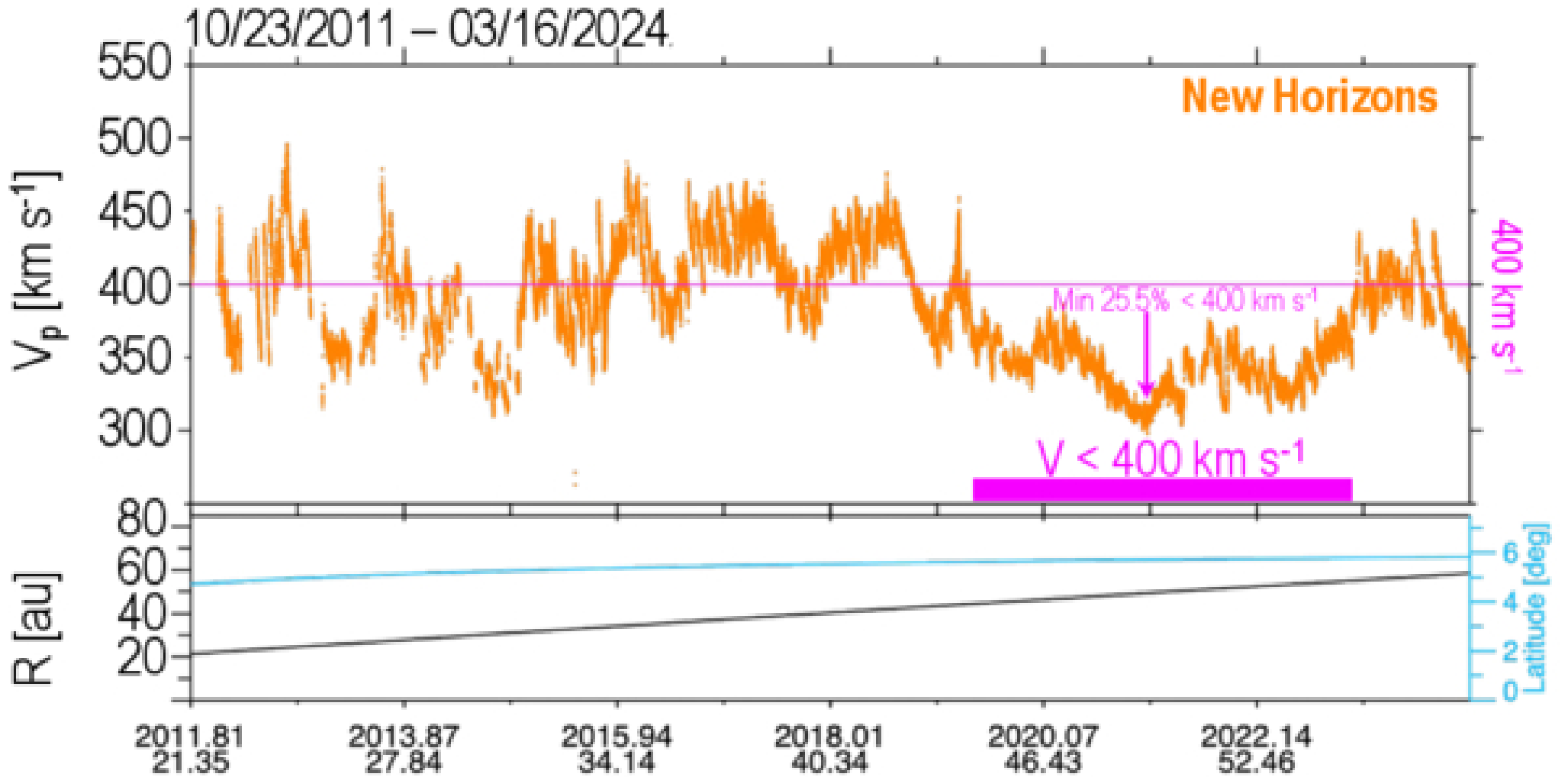
Figure 2. from Heather A. Elliott et al 2026 Astrophys. J. 1001 doi:10.3847/1538-4357/ae39c6 https://dx.doi.org/10.3847/1538-4357/ae39c6 © 2026. The Author(s). Published by the American Astronomical Society.
