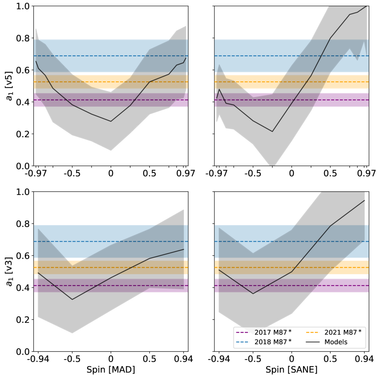
Figure 9. from Vadim Bernshteyn et al 2026 Astrophys. J. 1000 doi:10.3847/1538-4357/ae34af https://dx.doi.org/10.3847/1538-4357/ae34af © 2026. The Author(s). Published by the American Astronomical Society.
